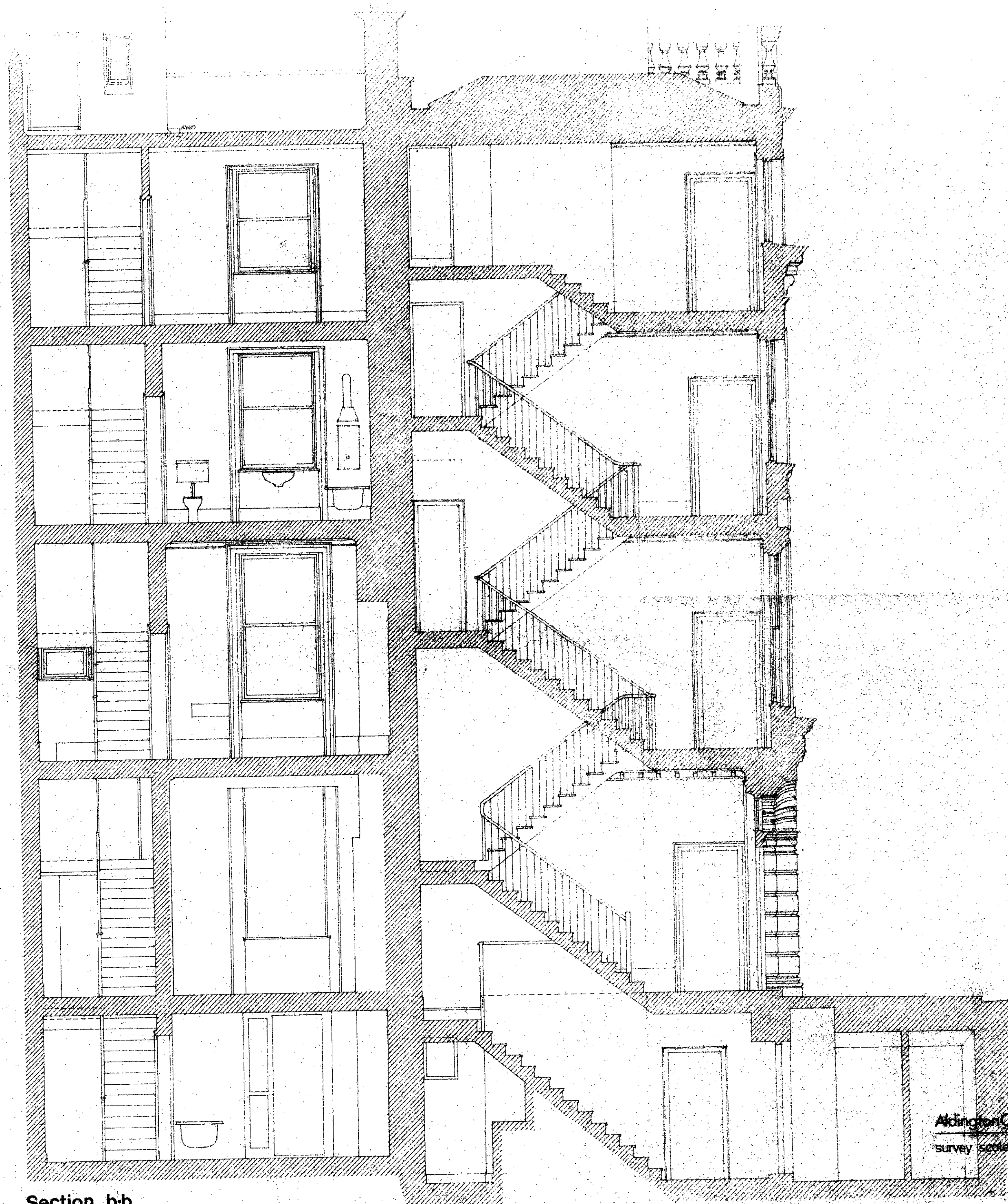
Section b-b
