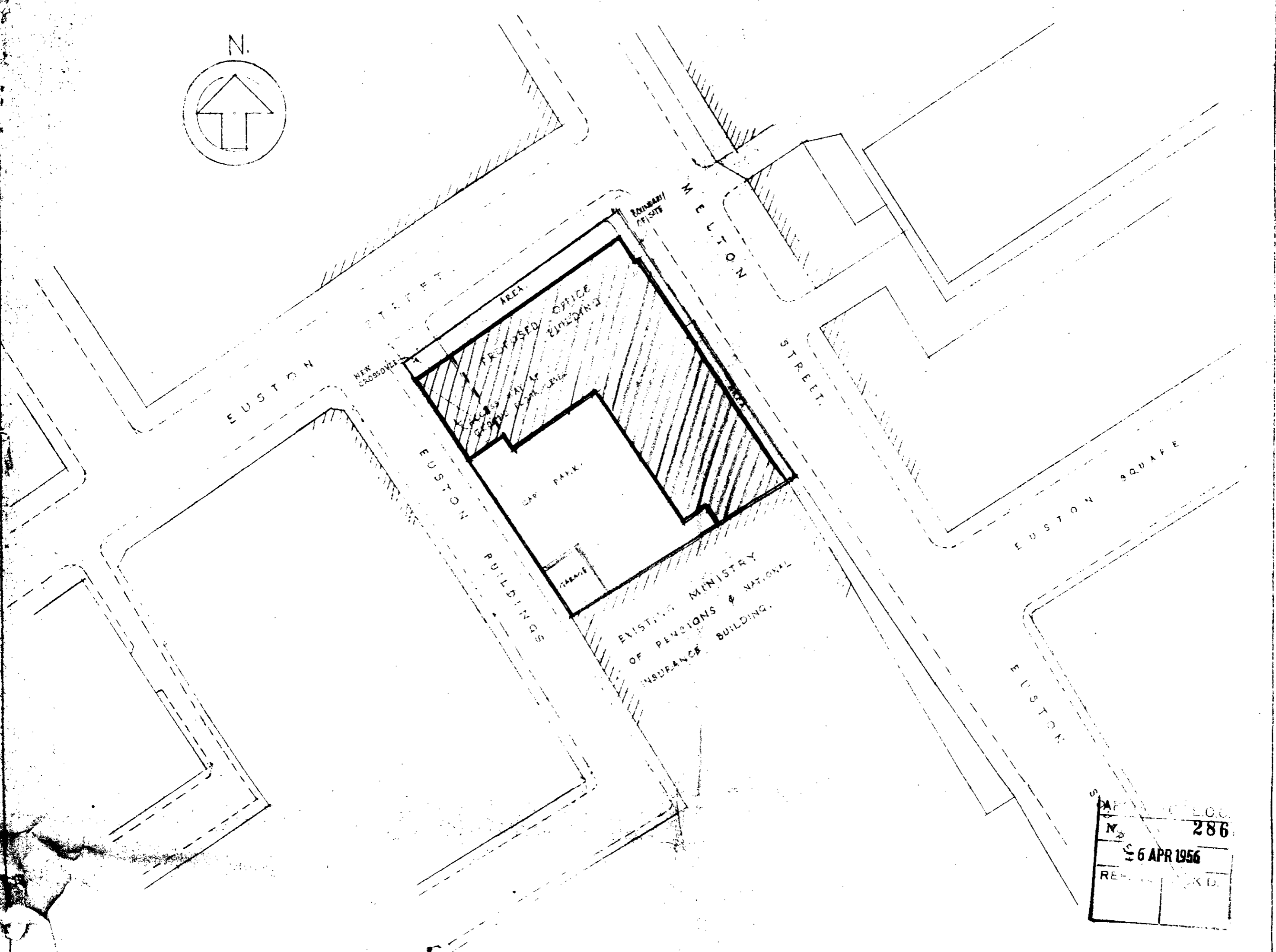
DRAWING No 236/168 SCALE: 32 FEET TO 1 INCH DECEMBER 1955. 3-10 MELTON STREET, 54-65 EUSTON STREET, & 1-11 EUSTON BUILDINGS. BLOCK PLAN SHOWING PROPOSED DEVELOPMENT. WALTER W. FICK, S.A. (L.C.C.) SIDNEY B. FICK, S.A. (L.C.C.) CHARTERED ARCHITECTS, 24 BUCKINGHAM STREET, STRAUD, LONDON W.C.2
