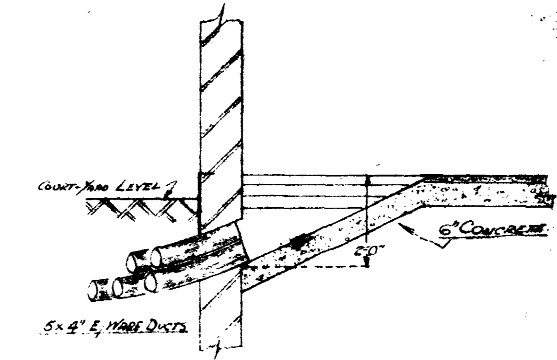
SECTION BB
