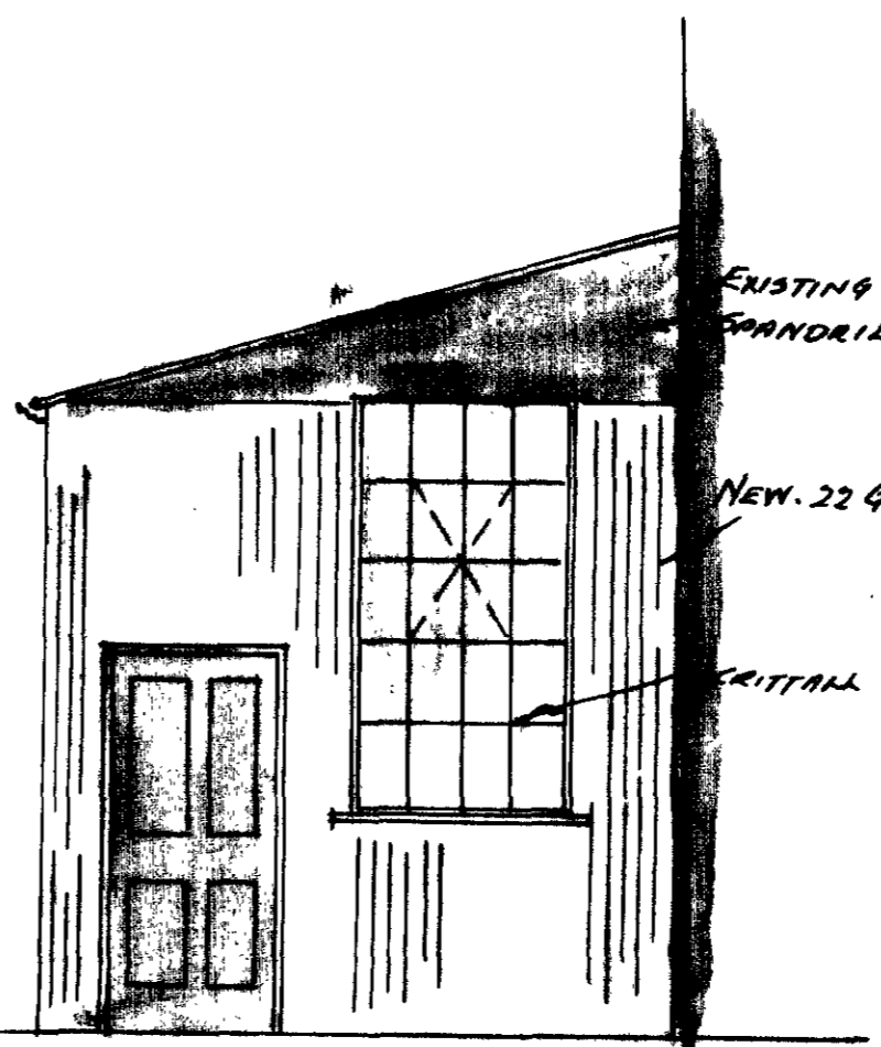
SIDE ELEVATION.
