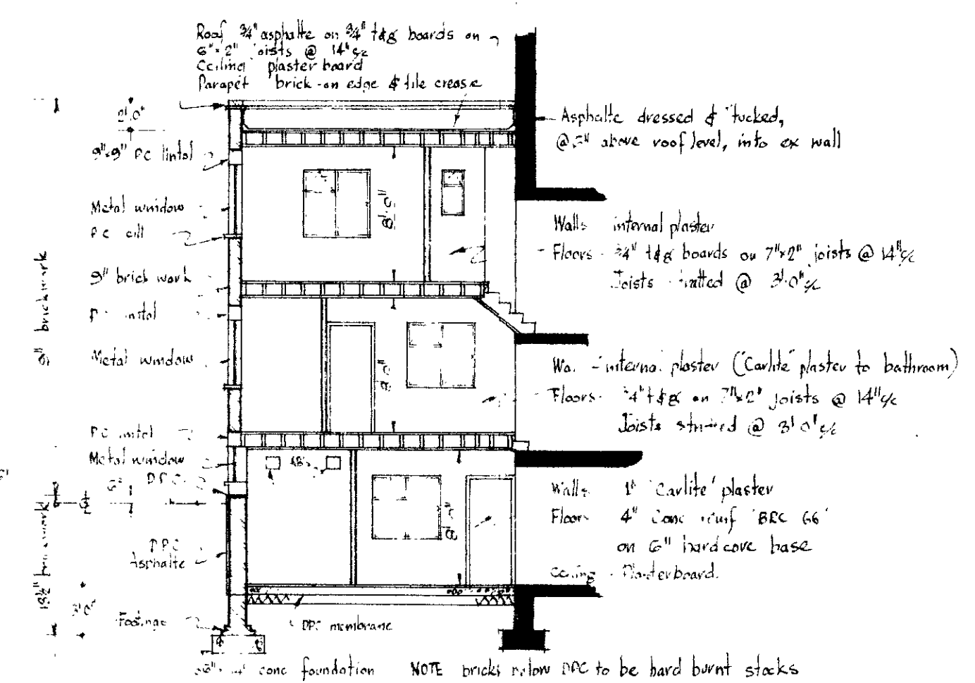
SECTION THRO' EXTENSION
