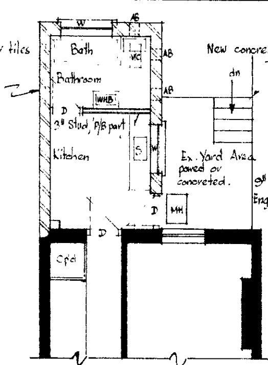
BASEMENT
