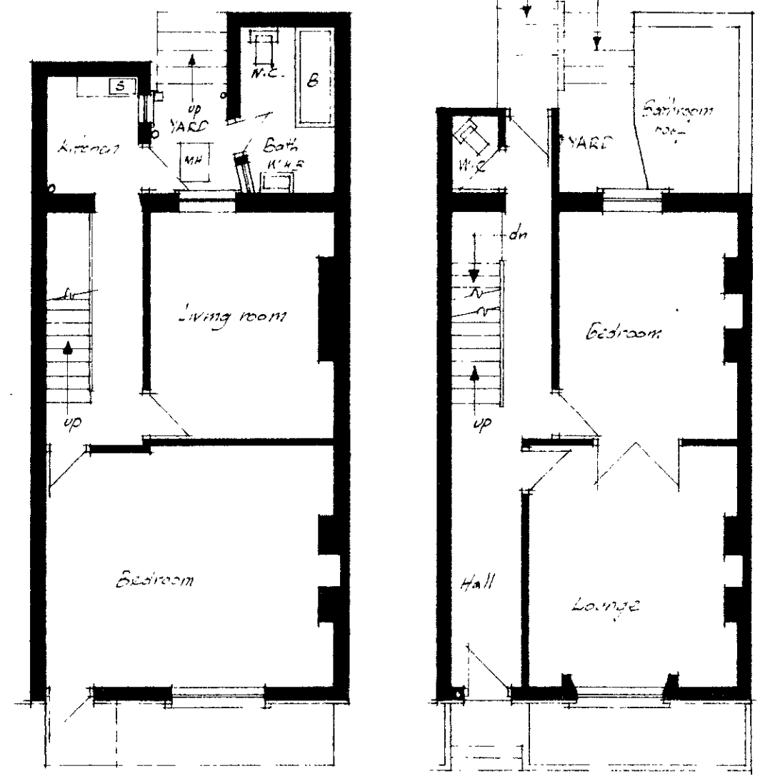
BASEMENT
