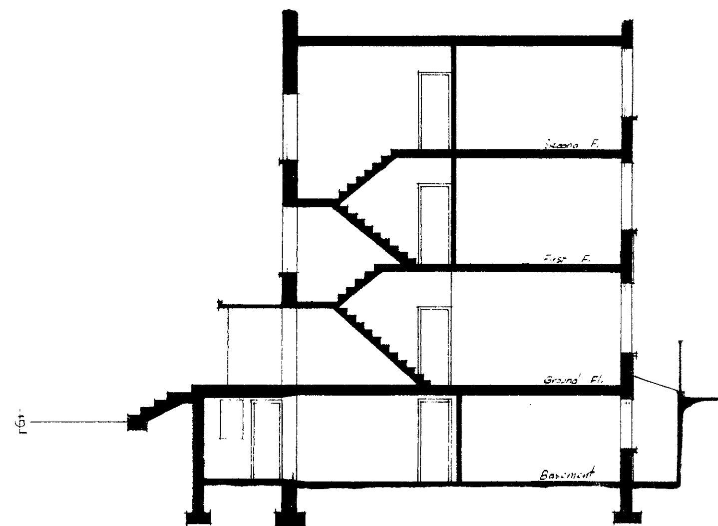
EXISTING SECTION
