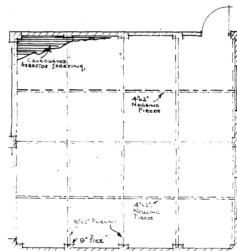
PLAN OF ROOF.
