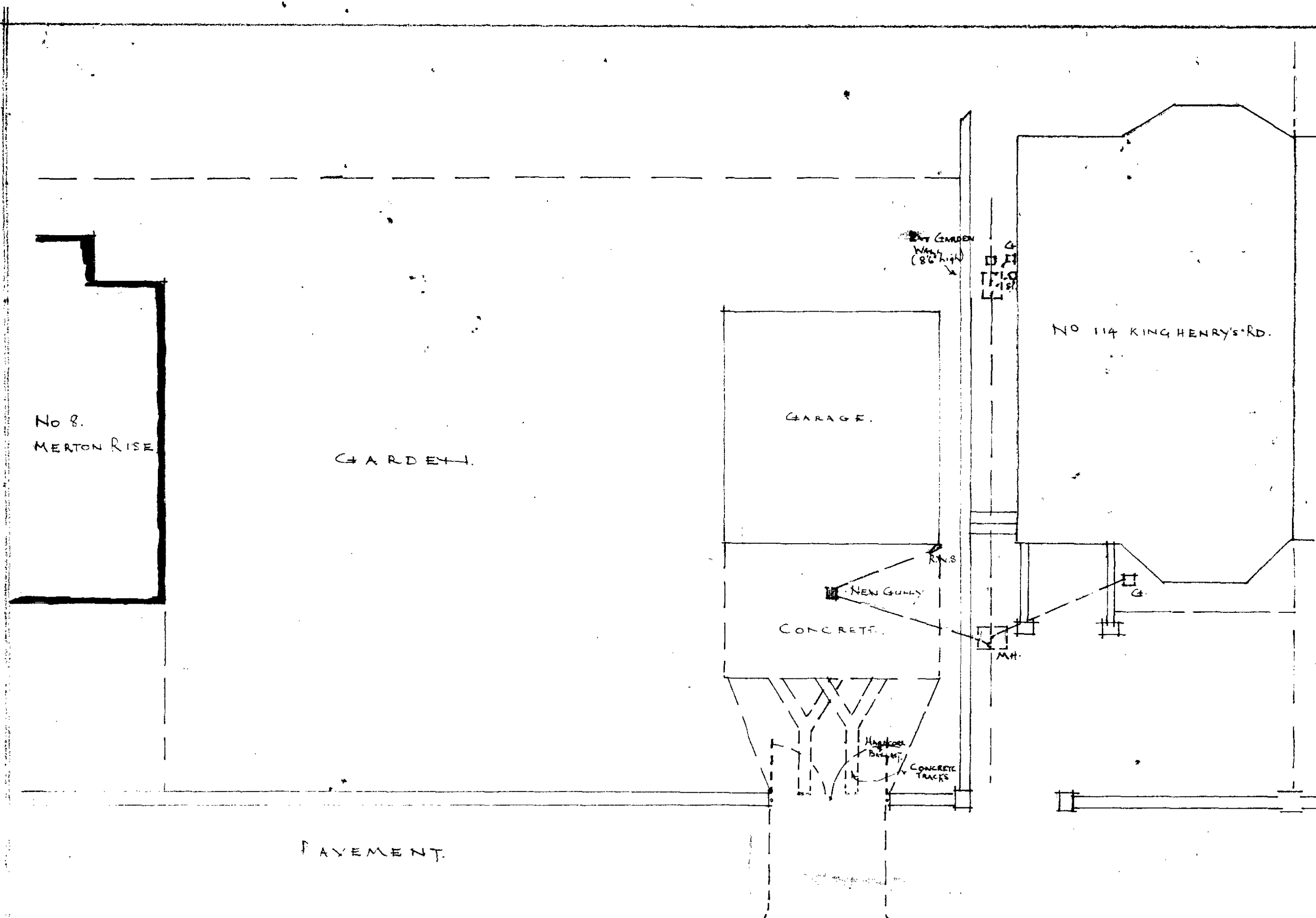
PLAN SHOWING NEW DRAINAGE. (SCALE 1/8" = ONE FOOT)
