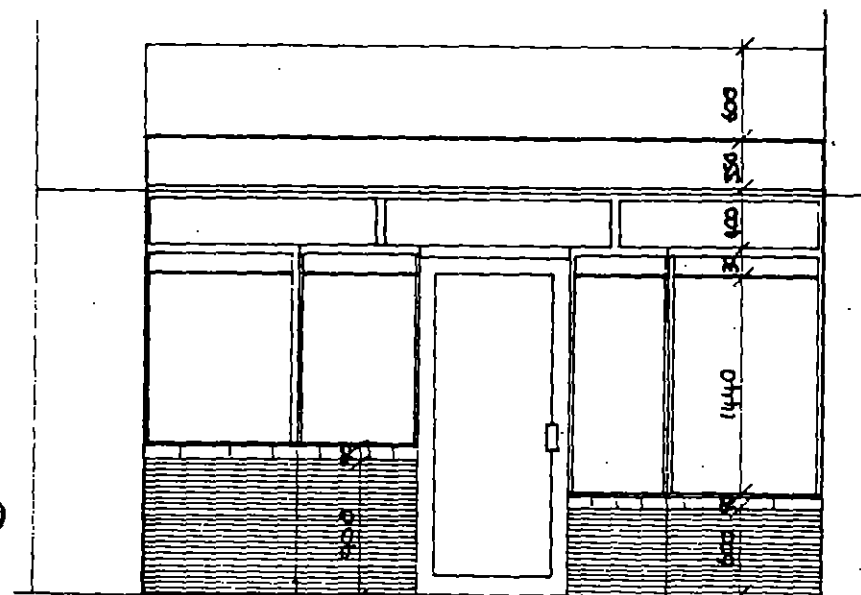
EXISTING ELEVATION
