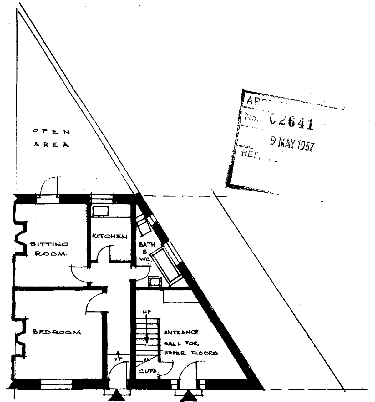
GROUND FLOORS
