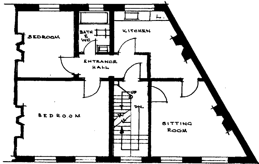
FIRST FLOORS
