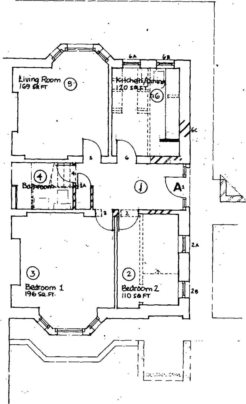
LOWER GROUND FLOOR : TWO BEDROOM UNIT
