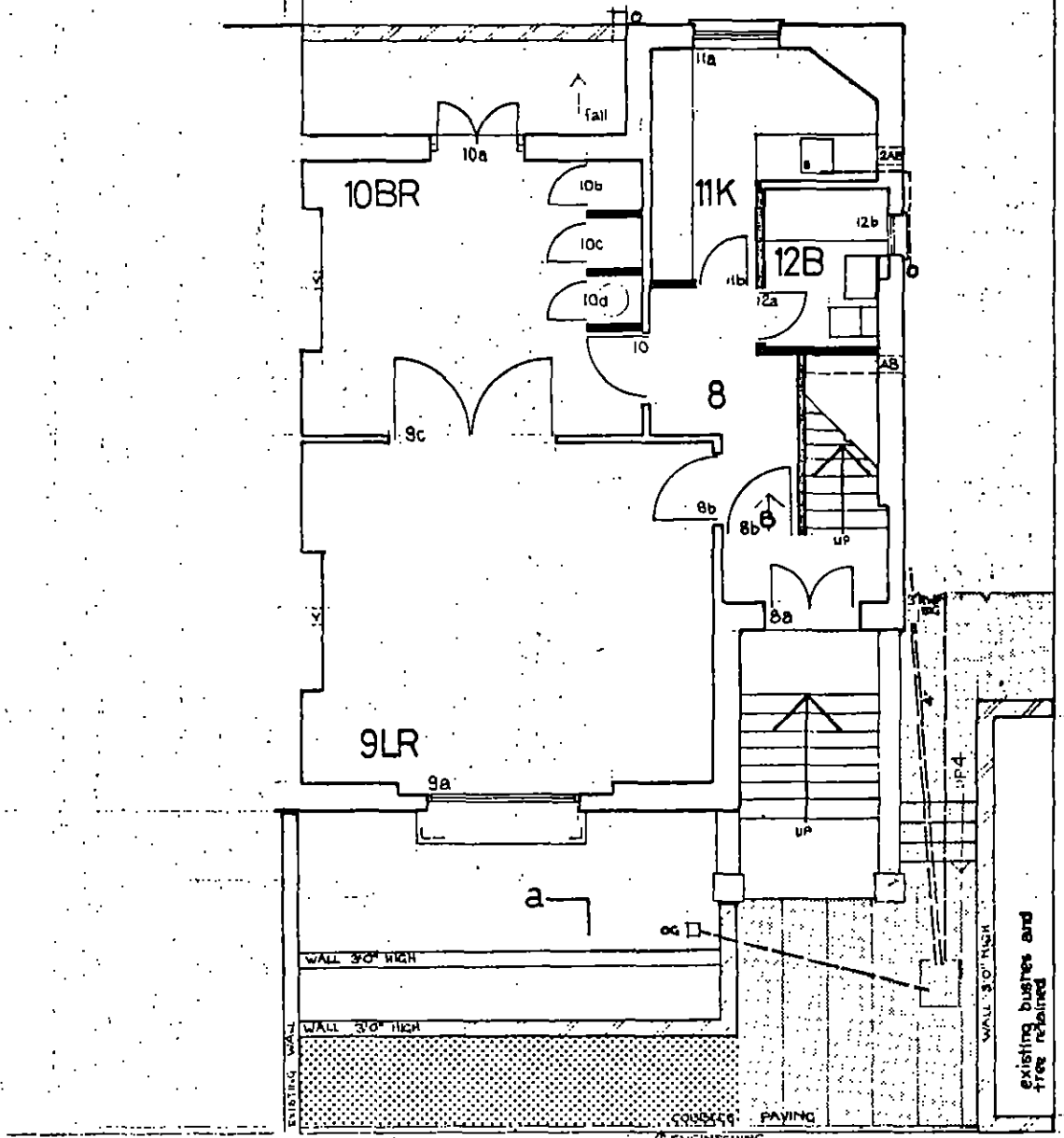
a Ground Floor
