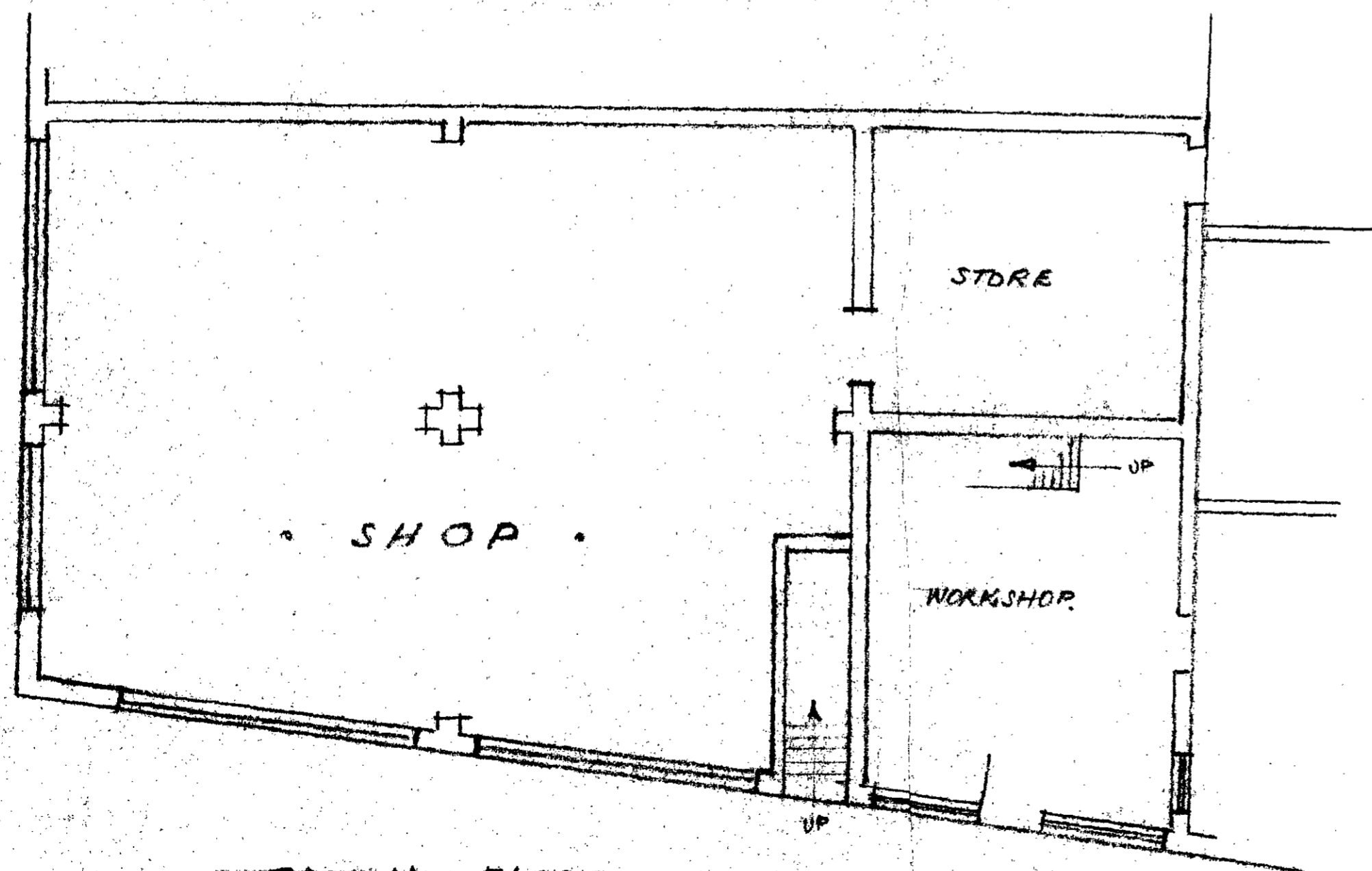
• GROUND FLOOR •
