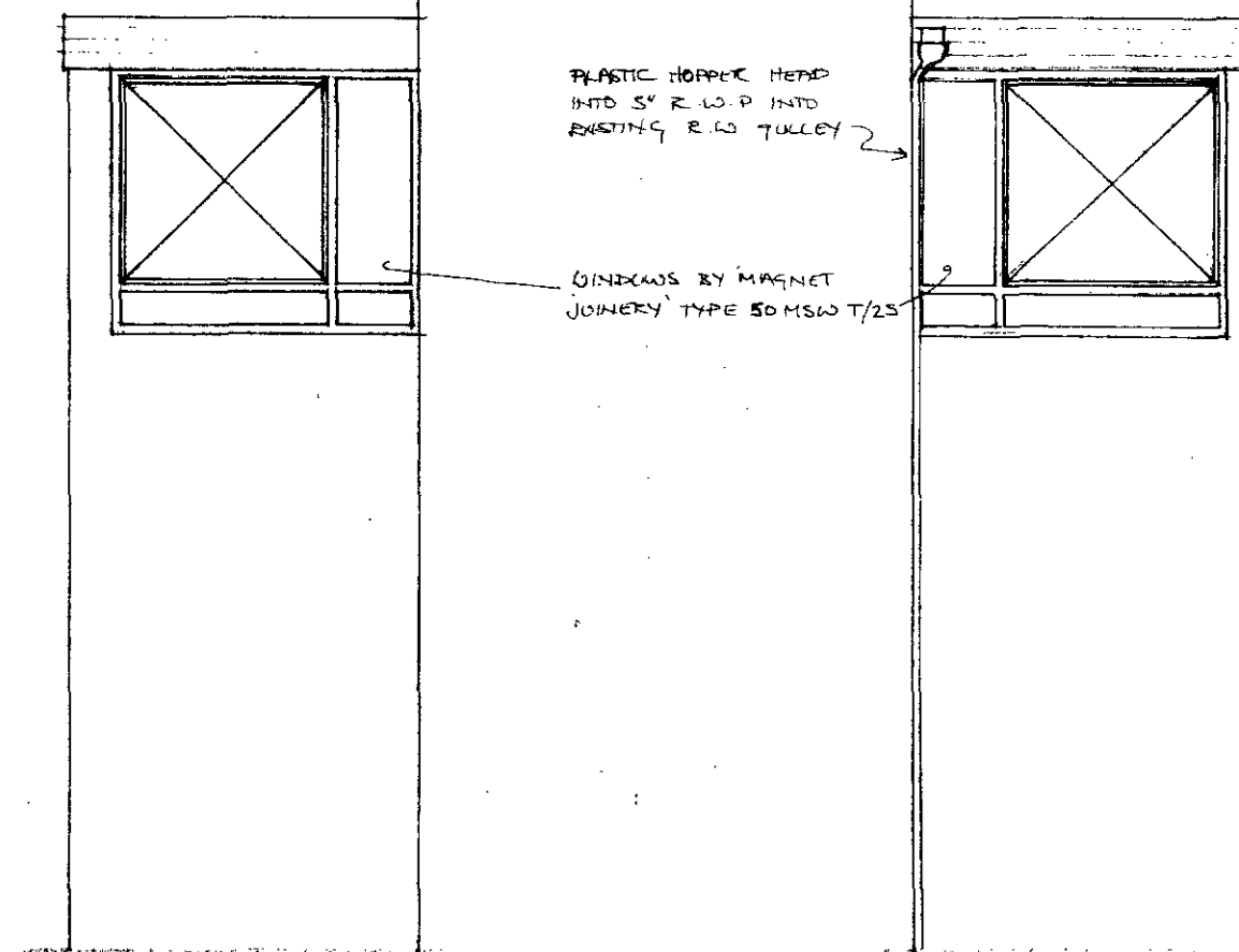
FLANK ELEVATIONS
