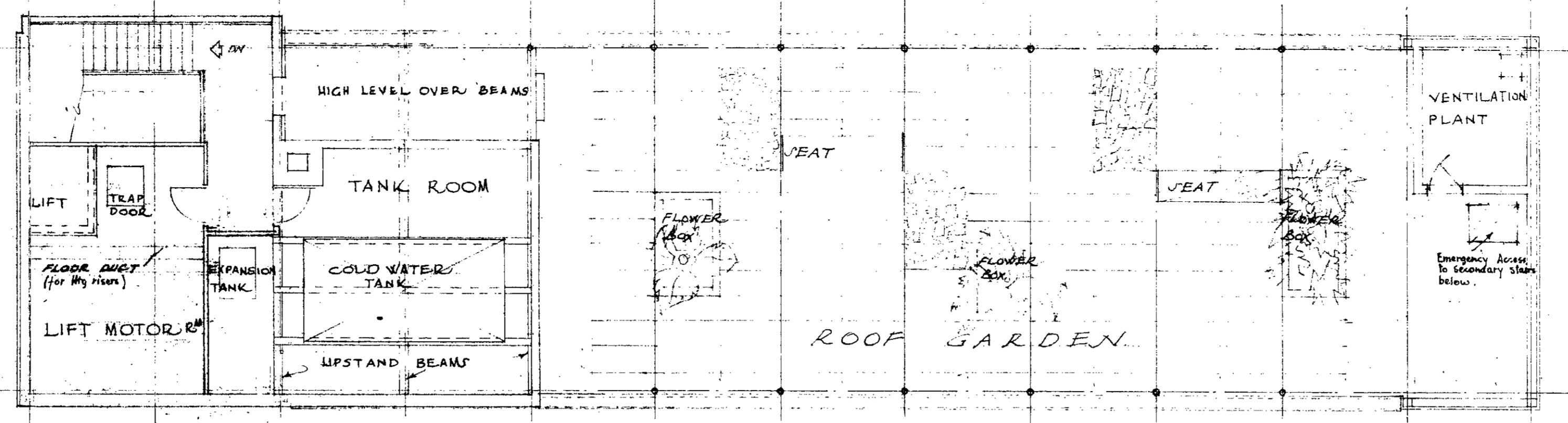
ROOF PLAN
