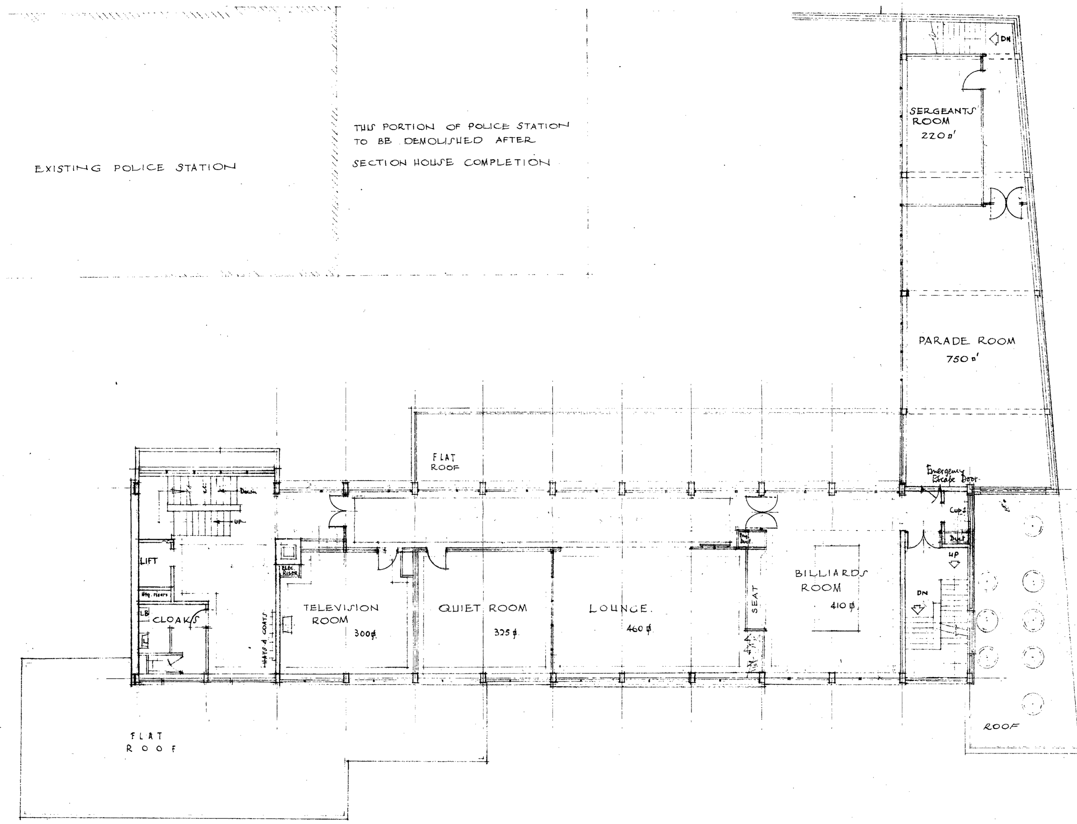
▪ FIRST FLOOR PLAN ▪ ▪ SCALE EIGHT FEET TO ONE INCH ▪
