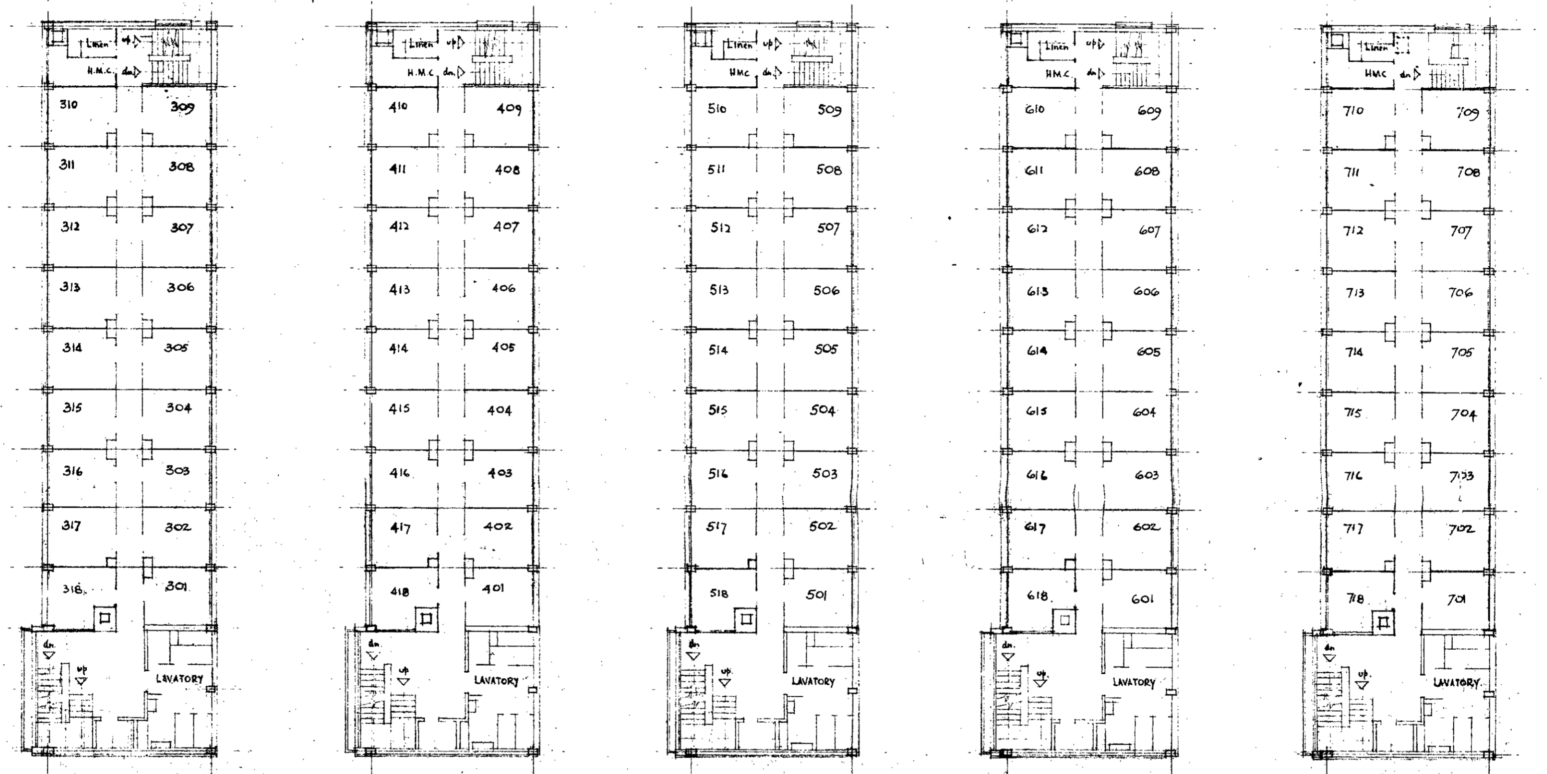
THIRD FLOOR FOURTH FLOOR FIFTH FLOOR SIXTH FLOOR SEVENTH FLOOR
