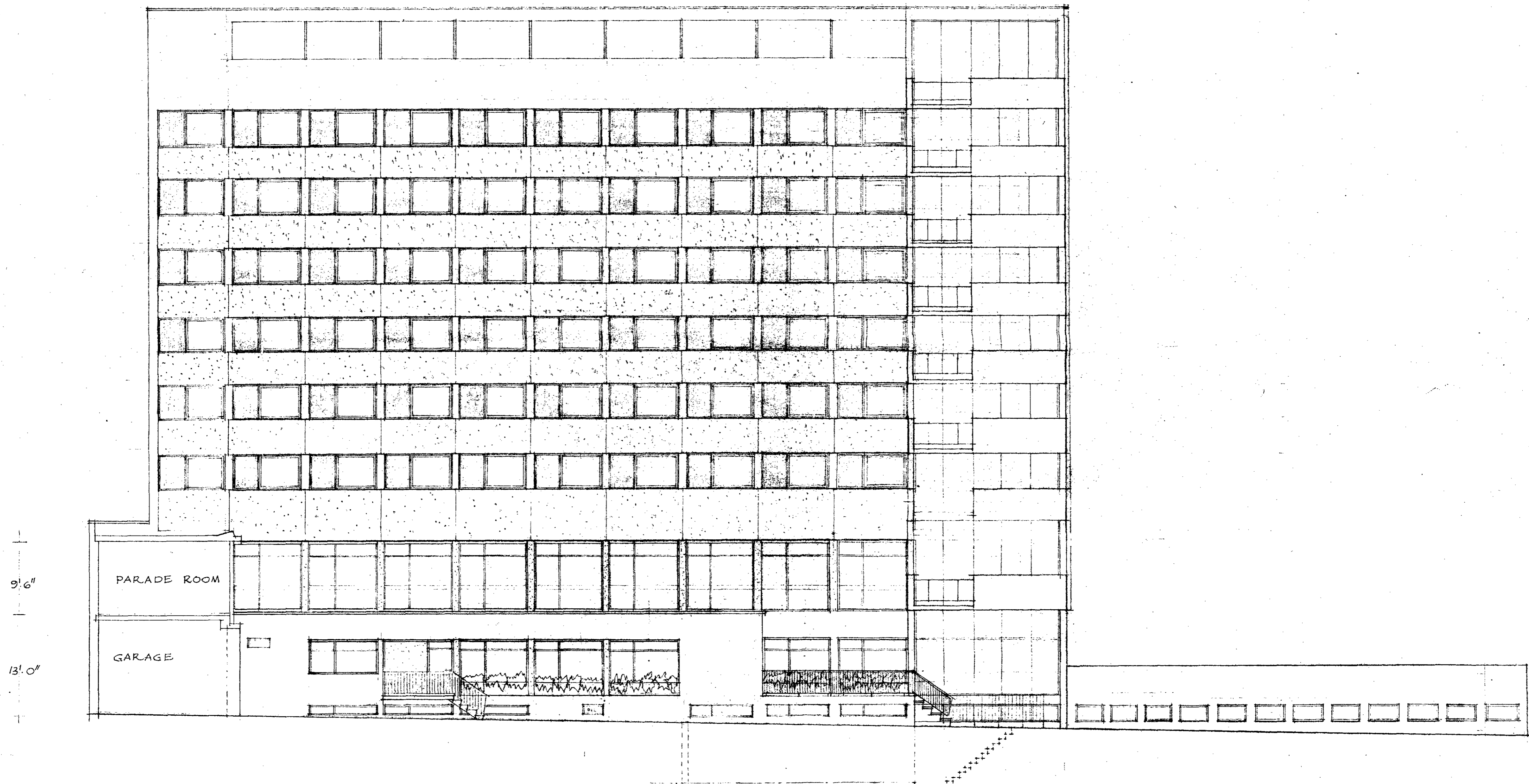
WEST ELEVATION SCALE EIGHT FEET TO ONE INCH
