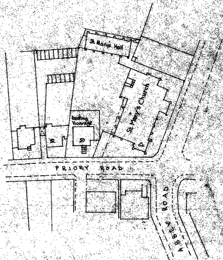
LOCATION PLAN SCALE 1/250th
