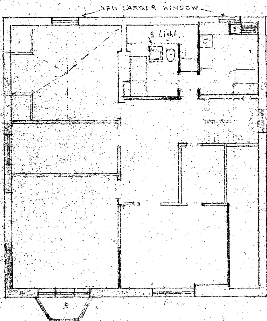
PROPOSED PLAN
