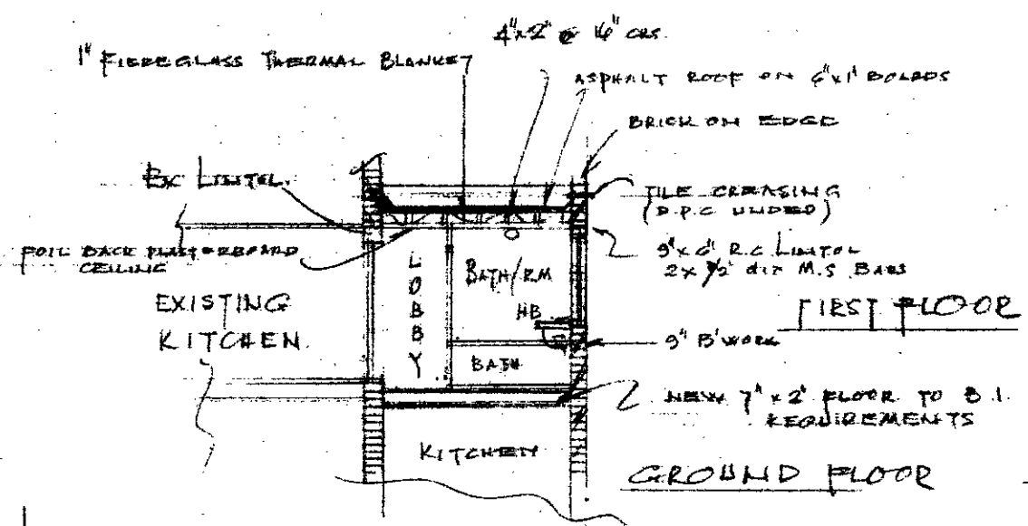
REAR SECTION 'A'
