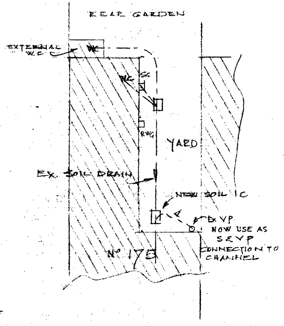
DRAINAGE PLAN GROUND LEVEL
