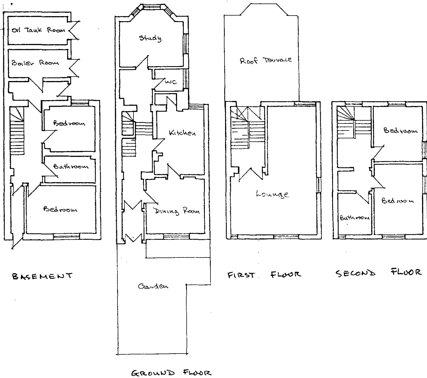
FLOOR PLANS AS EXISTING
