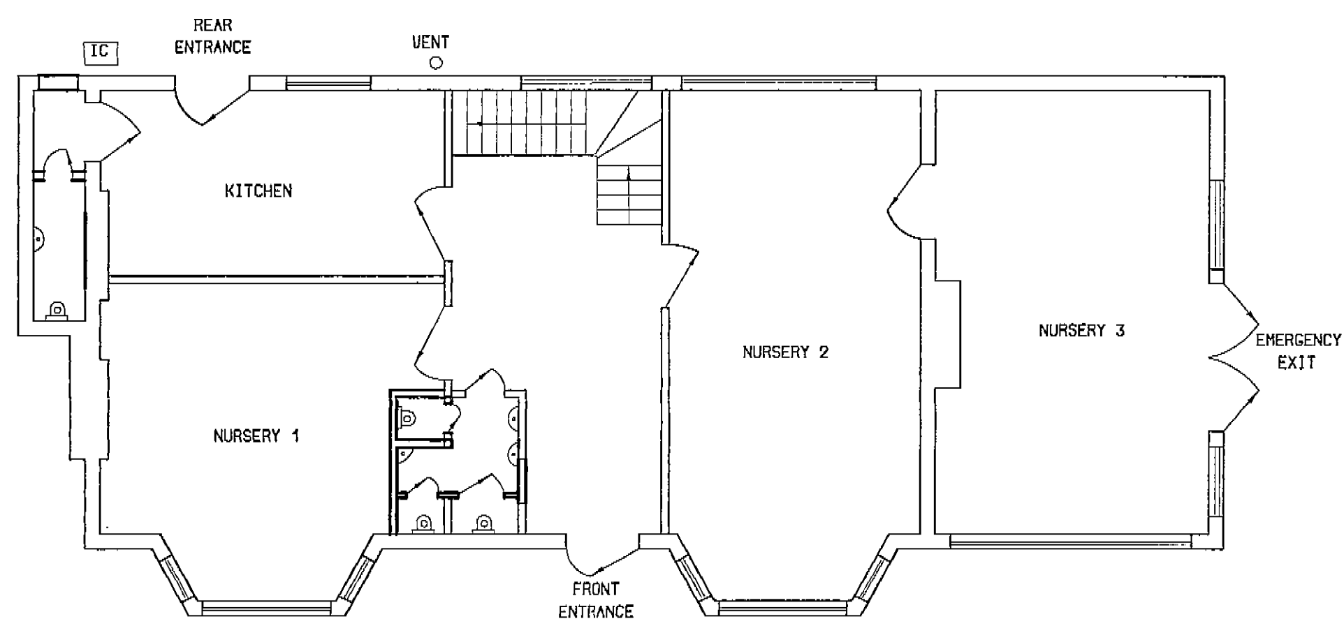
GROUND FLOOR
