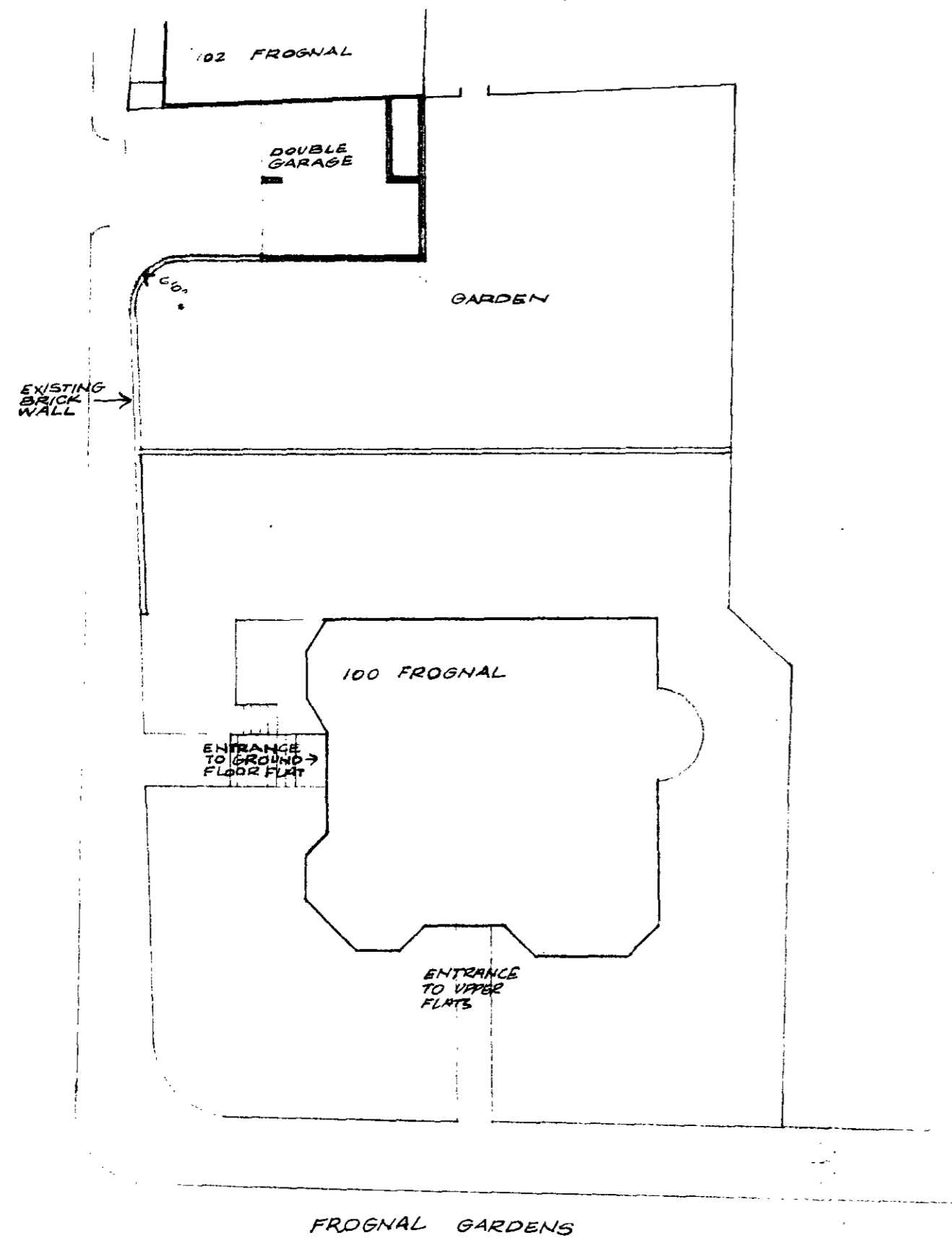
SITE PLAN SHOWING LAYOUT OF GARAGES SCALE 16 FEET TO ONE INCH
