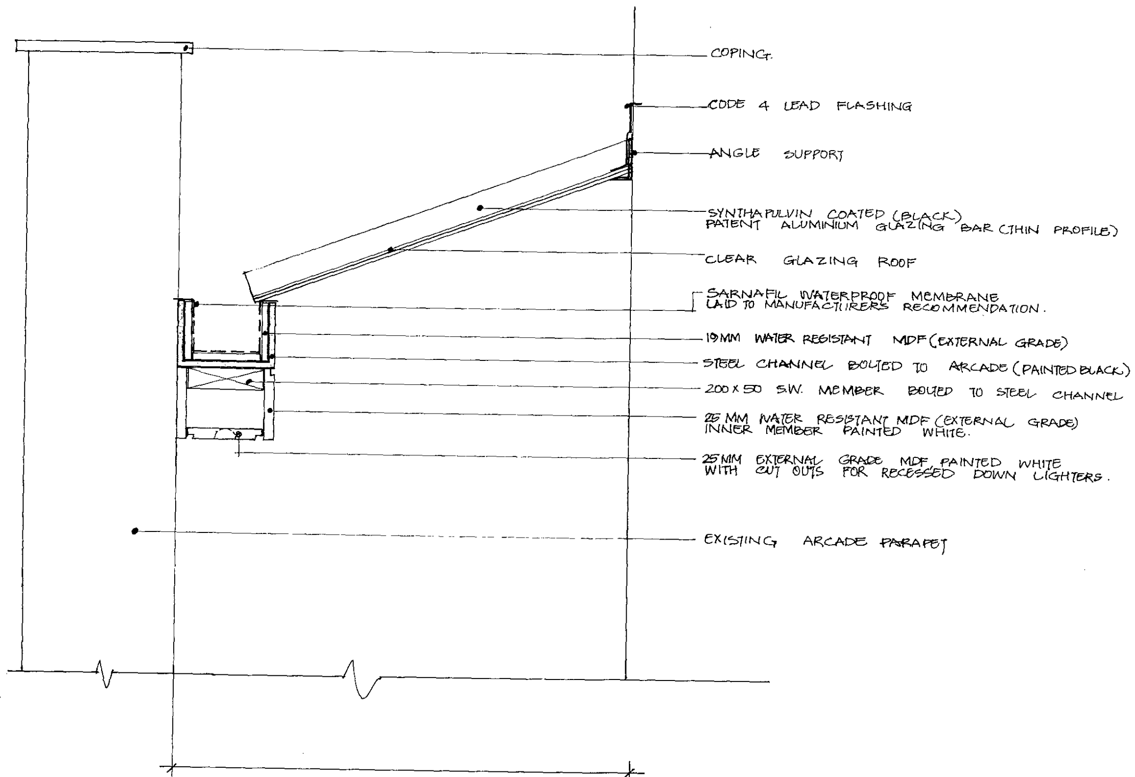
SECTION SCALE 1:10
