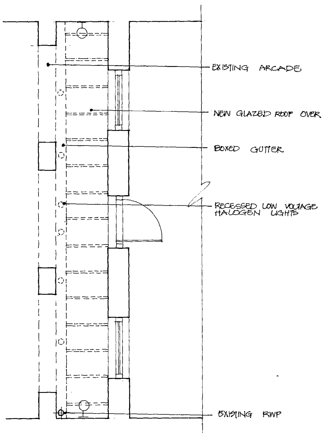
PLAN
