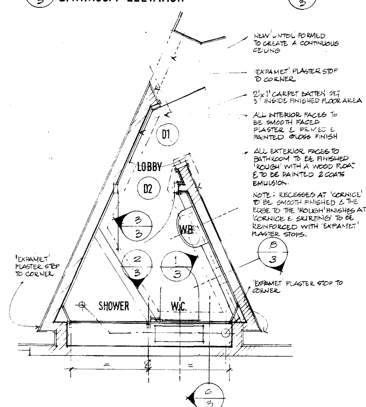
4 3 FLOOR PLAN OF BATHROOM
