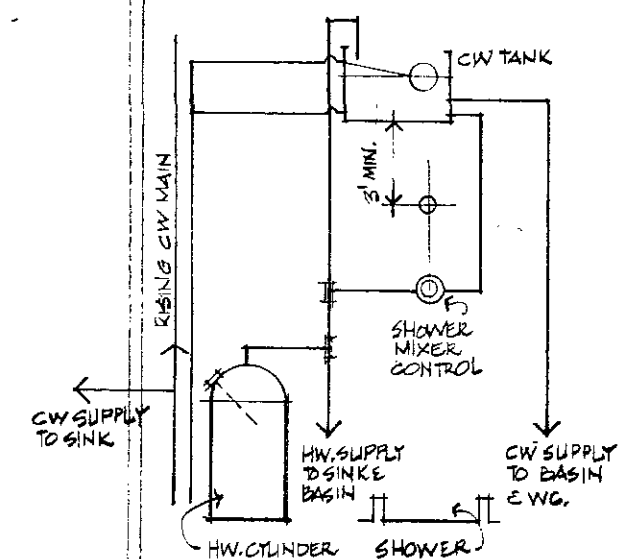
ARRANGEMENT OF PLUMBING SERVICES
