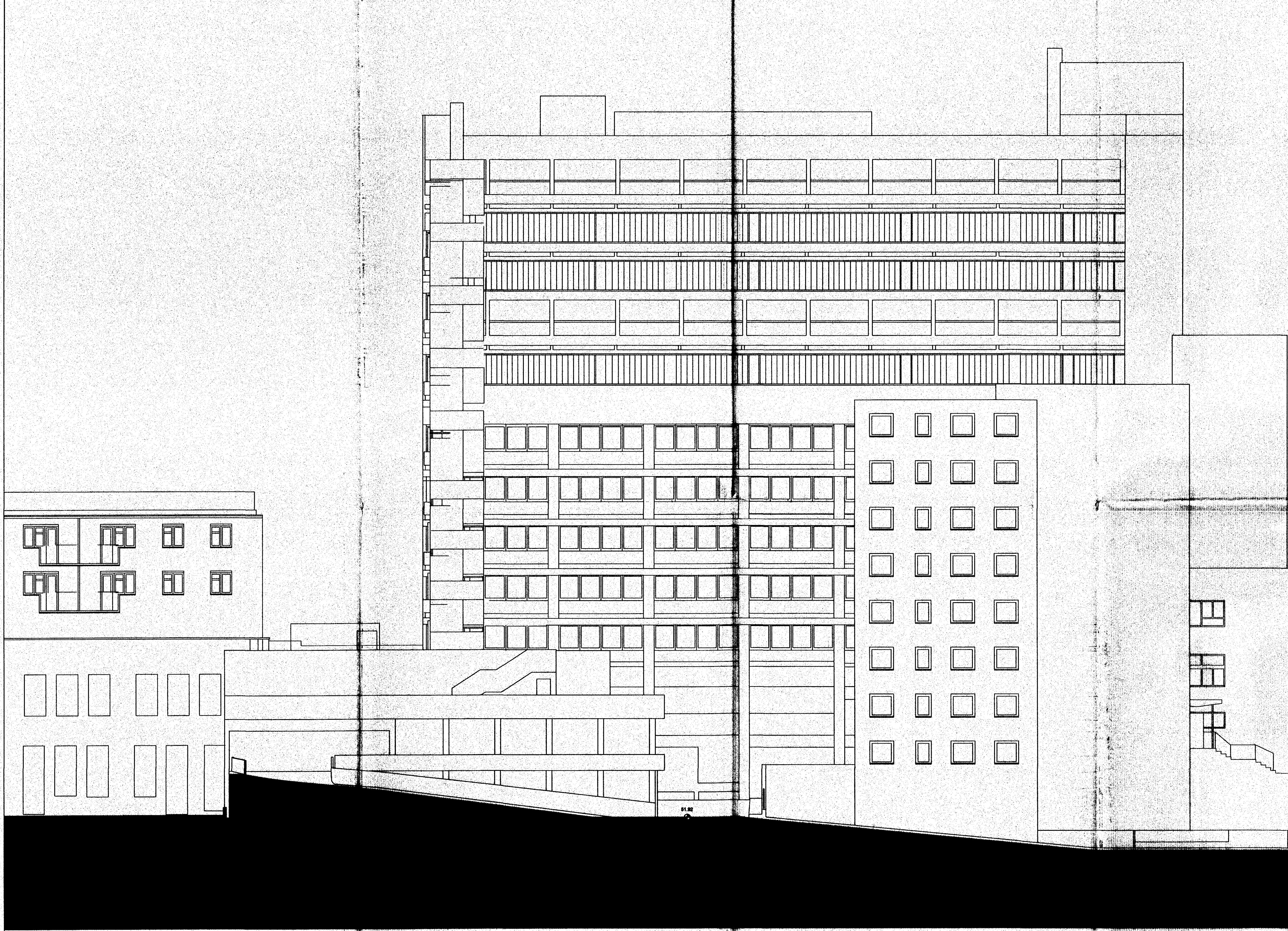
SECTION THROUGH CAR PARK RAMP
