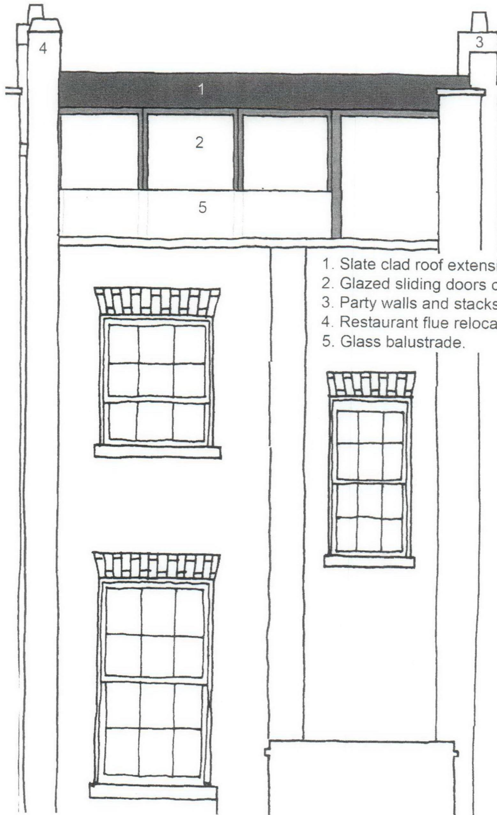
Rear elevation: as proposed scale 1:50
