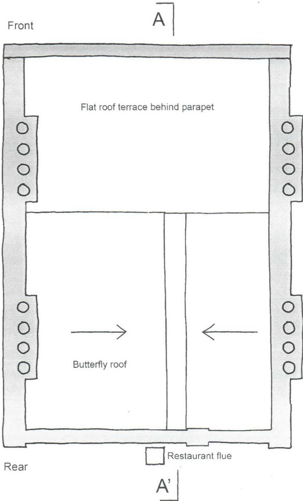
Roof plan: as existing scale 1:50
