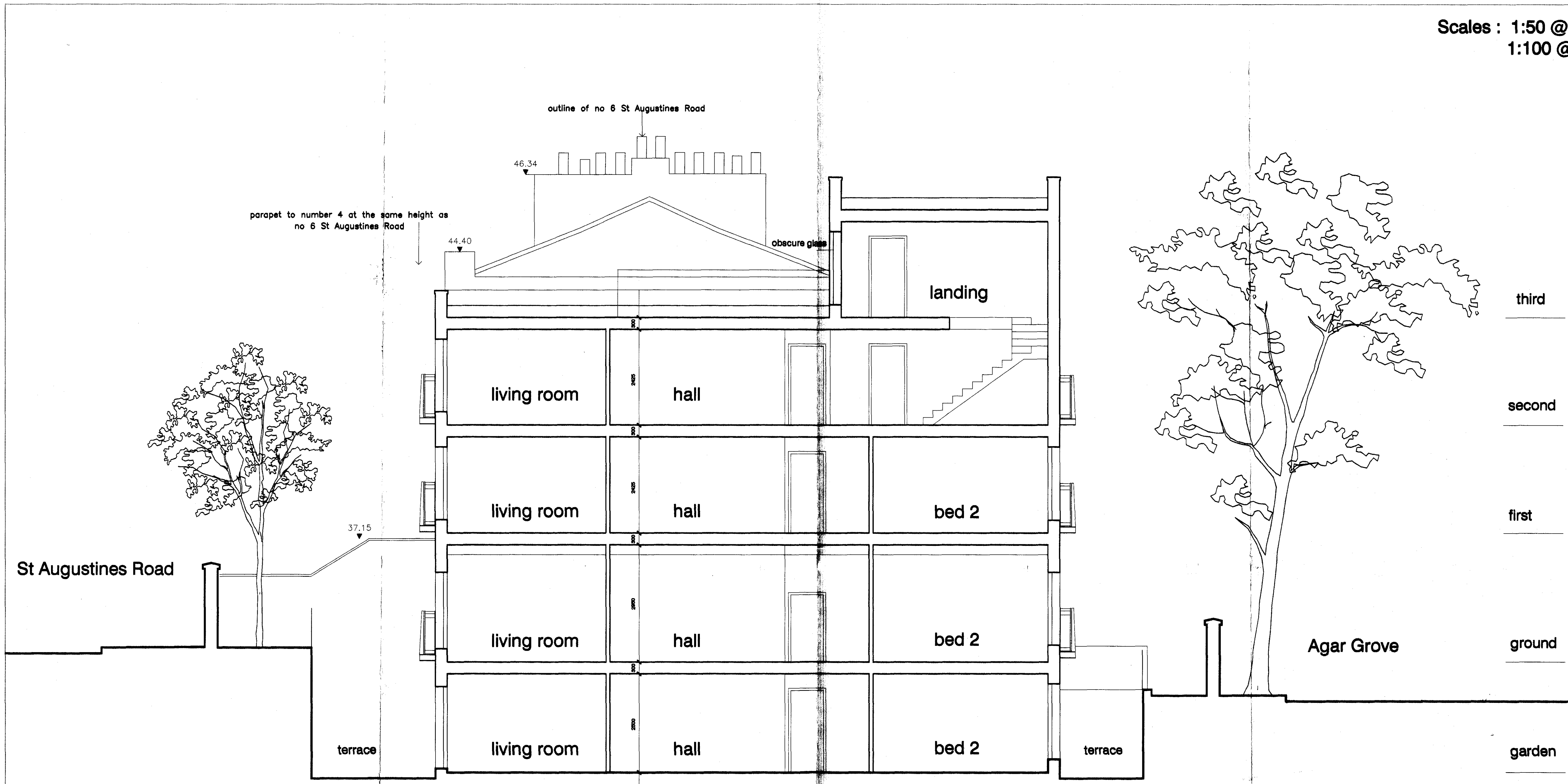
section AA looking towards 6 St Augustines Road
