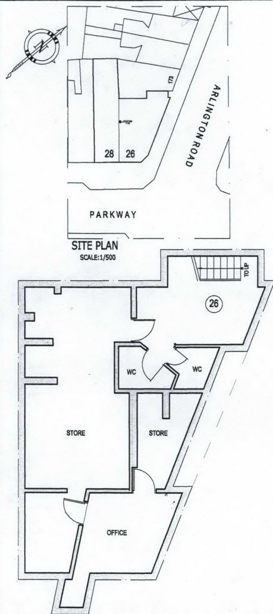
EXISTING BASEMENT FLOOR PLAN SCALE:1/100
