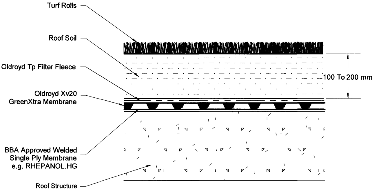
Turfed Roof
