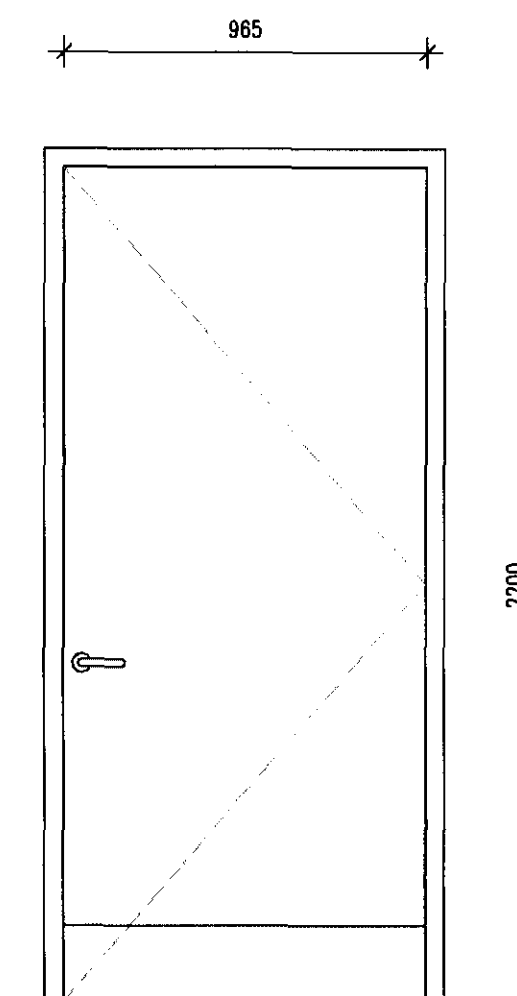
TYPE E TYPICAL LOCATION: TOILET / STORE
