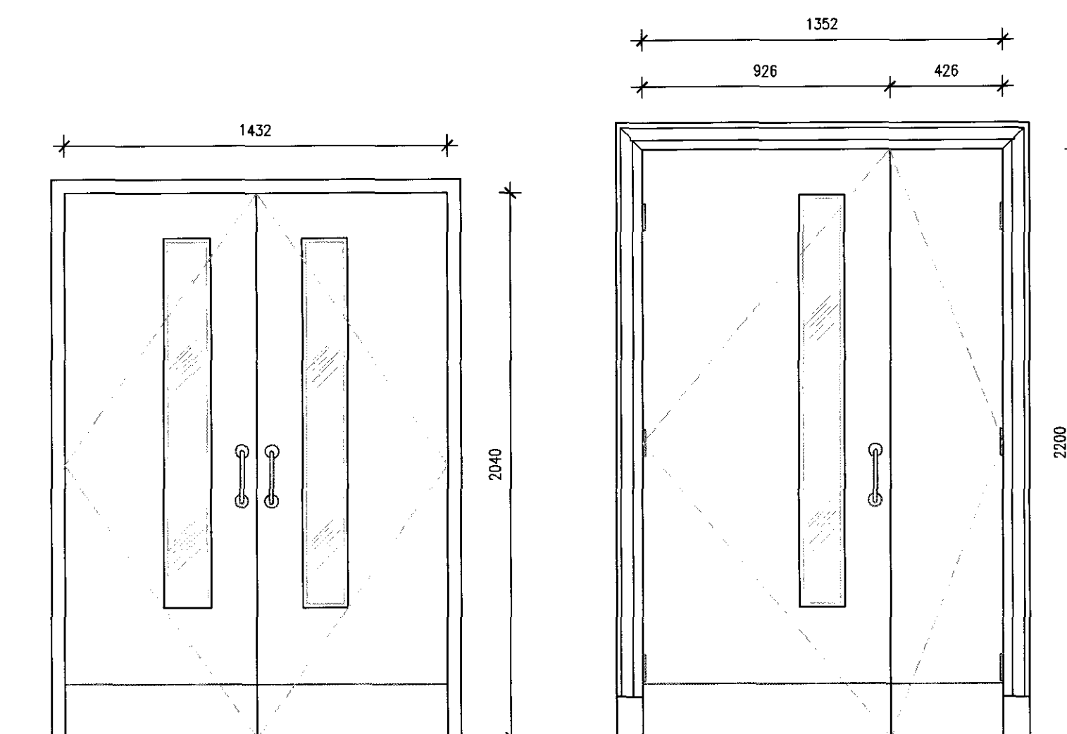
TYPE A TYPICAL LOCATION: EAST STAIRCASE
