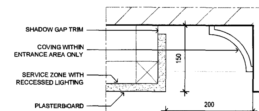
DETAIL AT EDGE OF PLASTERBOARD CEILING SCALE 1:5
