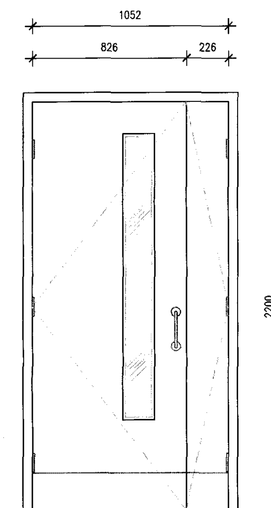
TYPE B2 TYPICAL LOCATION: MAIN STAIRCASE / CORRIDOR
