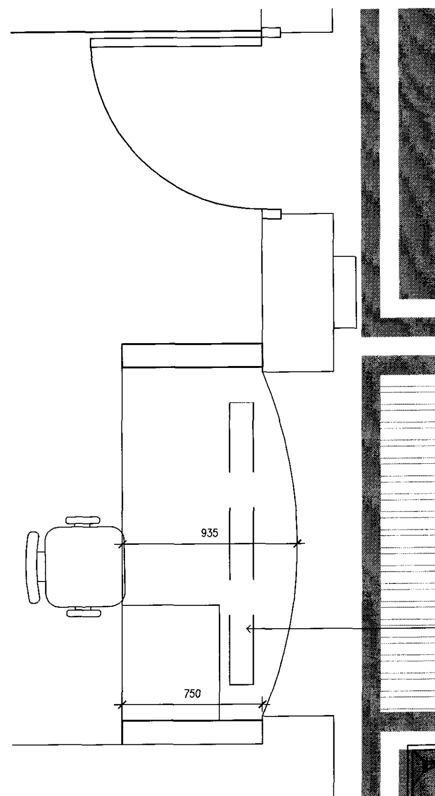
PLAN OF RECEPTION
