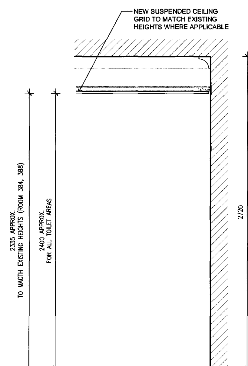
SECTIONS THROUGH CEILINGS
