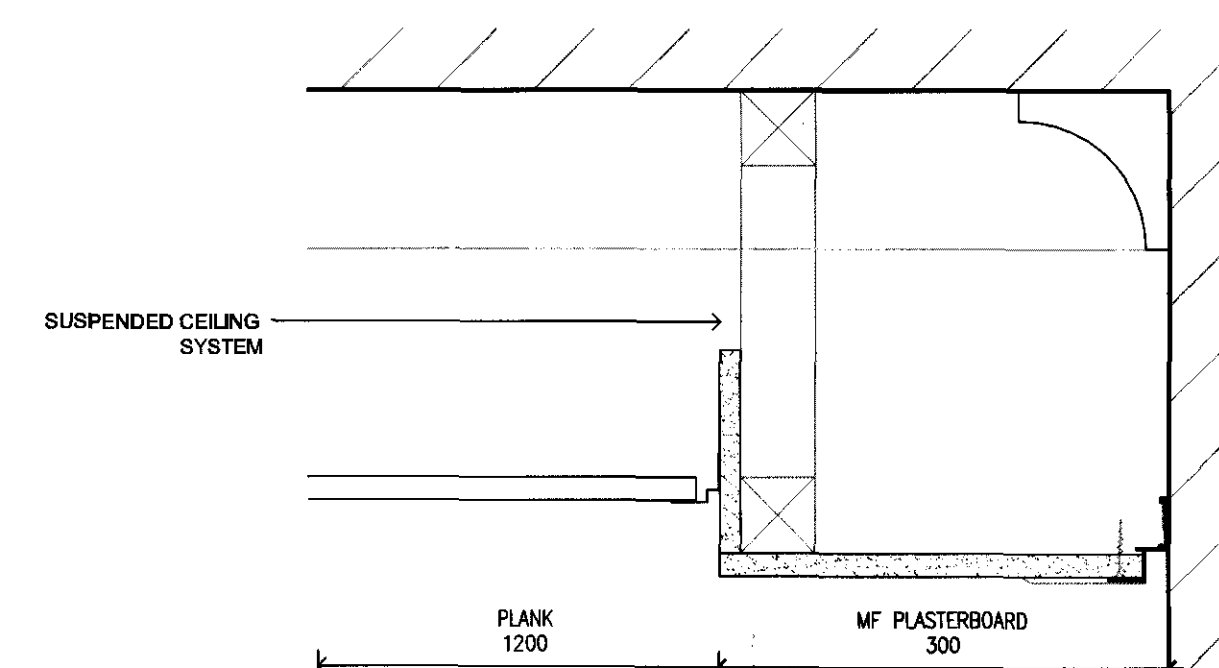
DETAIL AT EDGE OF CEILING - 3RD FLOOR CORRIDOR SCALE 1:5
