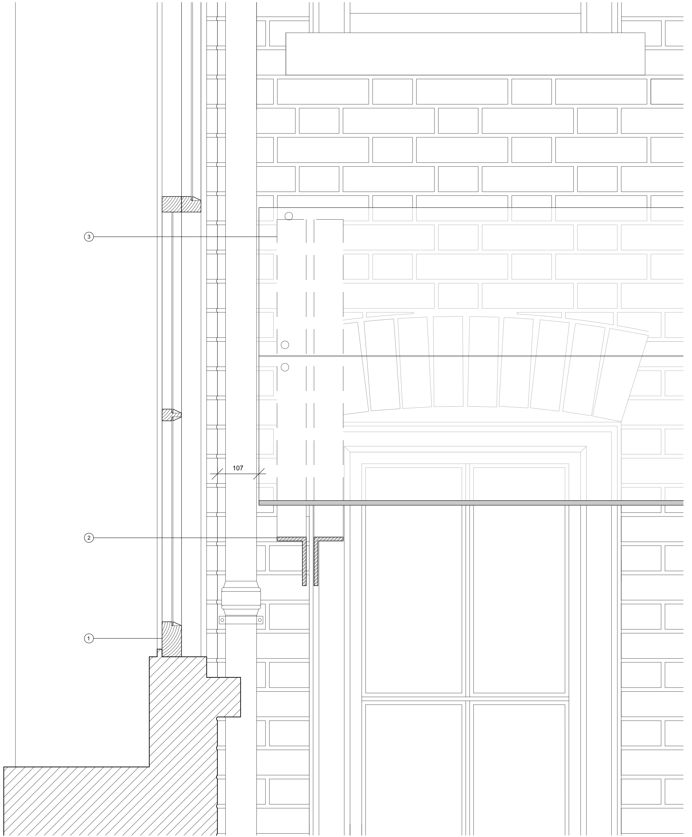
02 A(05)02 SECTION THROUGH EXISTING WINDOW AND PROPOSED GLAZED ROOF, SCALE 1:5
