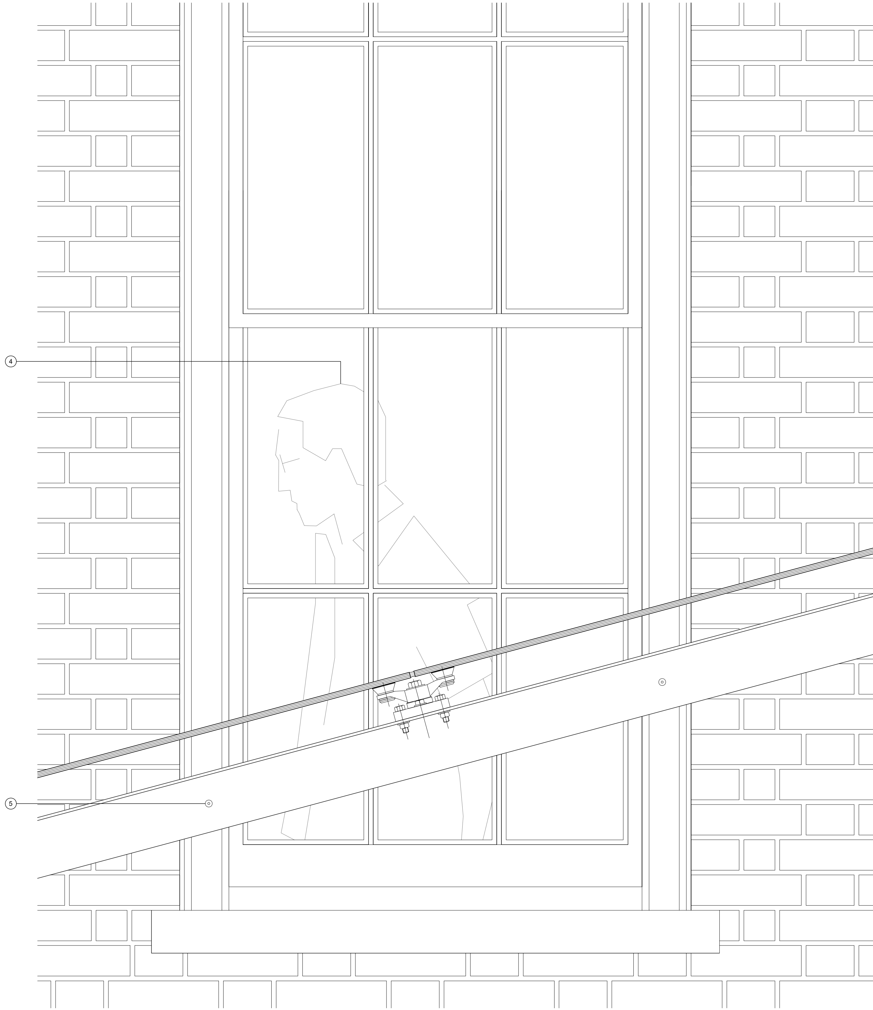
01 A(05)02 ELEVATION OF EXISTING WINDOW AND SECTION THROUGH PROPOSED GLAZED ROOF, SCALE 1:5
