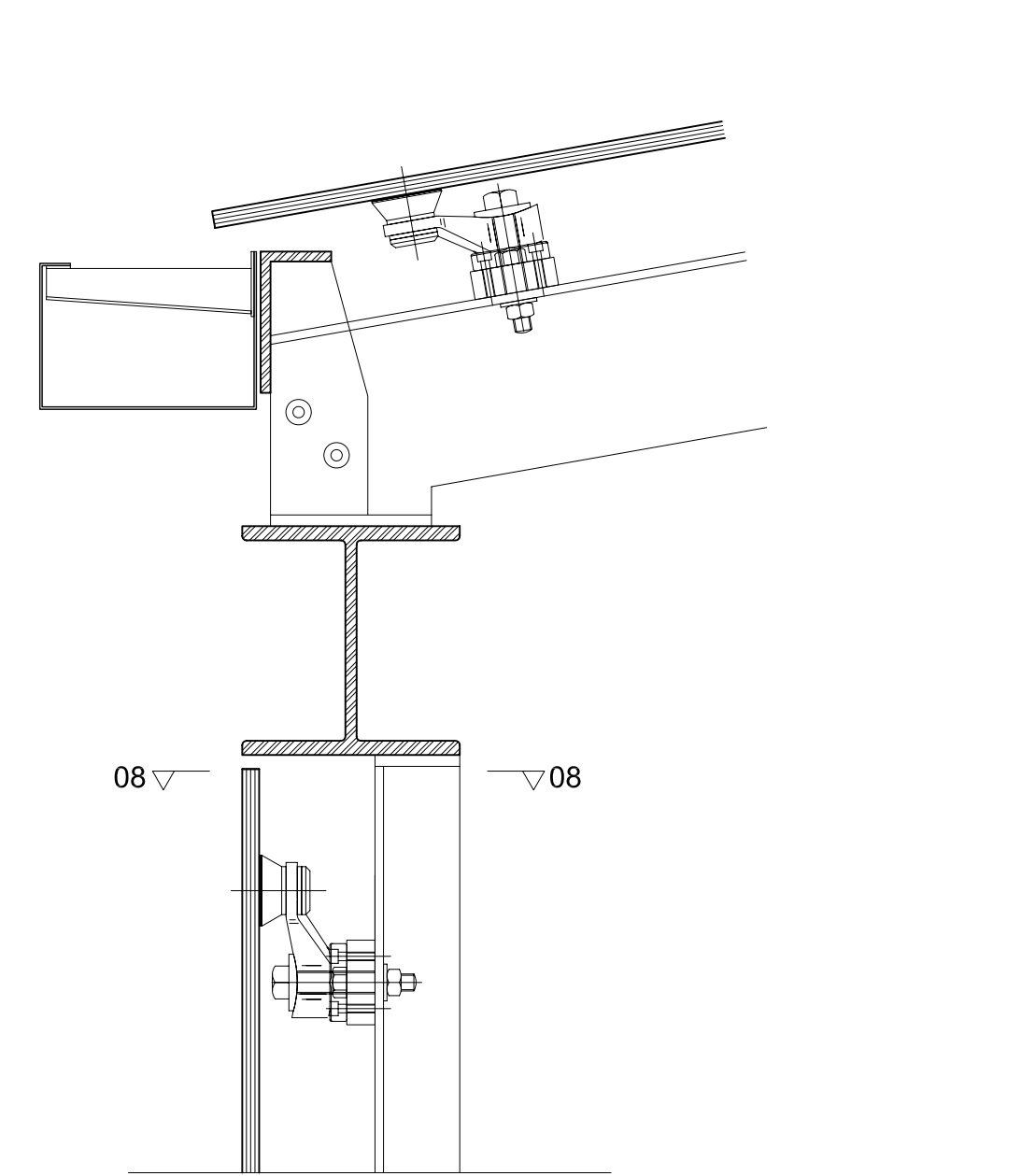
06 A(05)01 TYPICAL SECTION OF GLASS CANOPY WITH VERTICAL GLASS, SCALE 1:5
