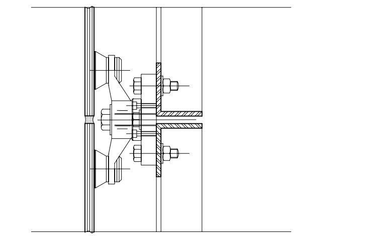
08 A(05)01 PLAN SECTION OF VERTICAL GLASS, SCALE 1:5
