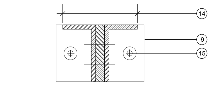
10 A(05)01 TYPICAL SECTION OF STEEL BEAM AND BRACKET TO BRICKWORK, SCALE 1:5
