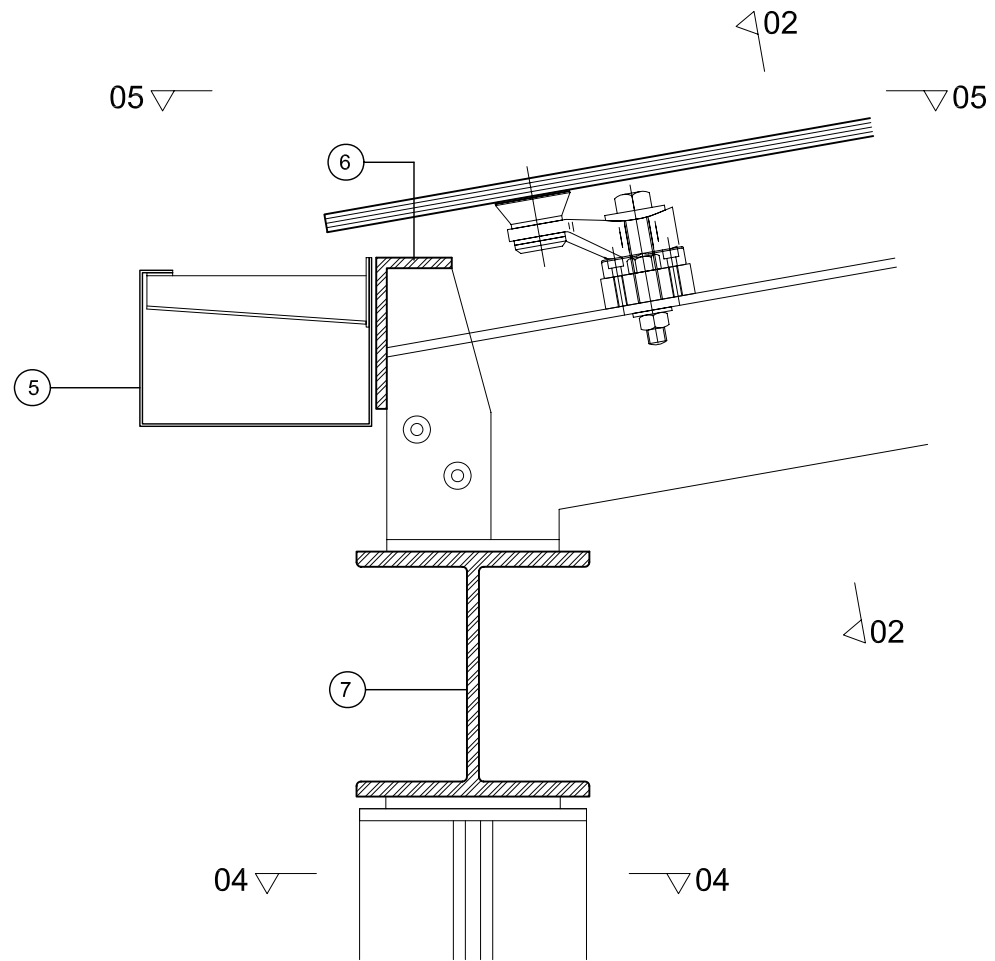
03 A(05)01 TYPICAL SECTION OF GLASS CANOPY, SCALE 1:5
