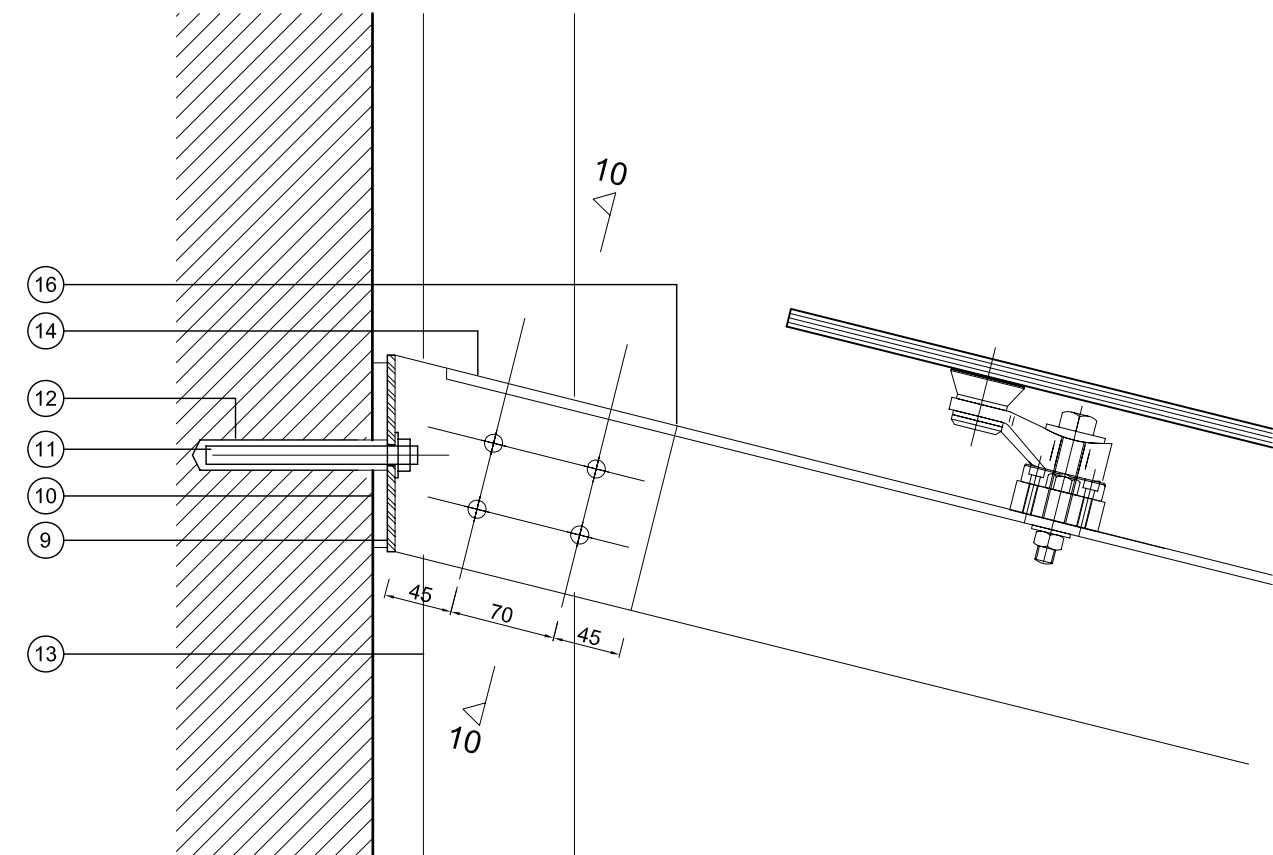
09 A(05)01 SECTION THROUGH CONNECTION TO BRICKWORK, SCALE 1:5
