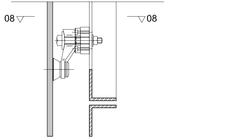
07 A(05)01 SECTION OF BASE OF VERTICAL GLASS, SCALE 1:5
