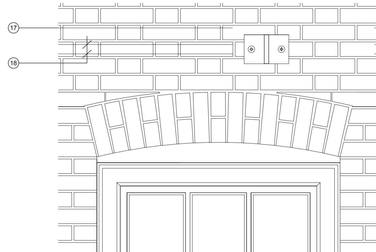
11 A(05)01 TYPICAL POSITION OF CONNECTION, SCALE 1:10
