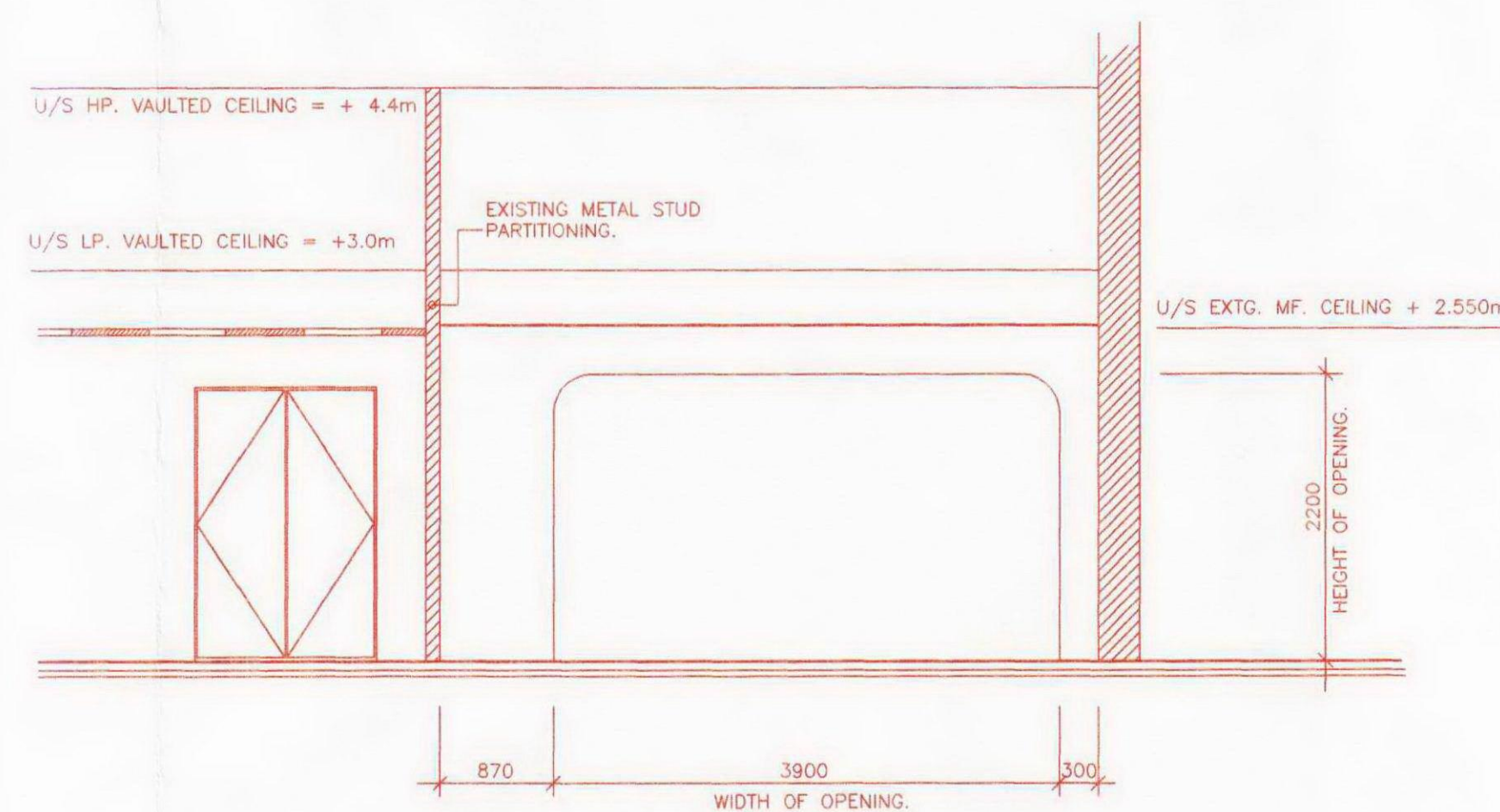
SECTION A - A 3.02
