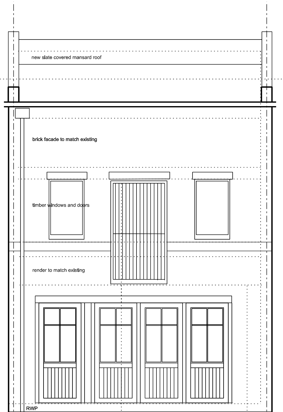
FRONT ELEVATION
