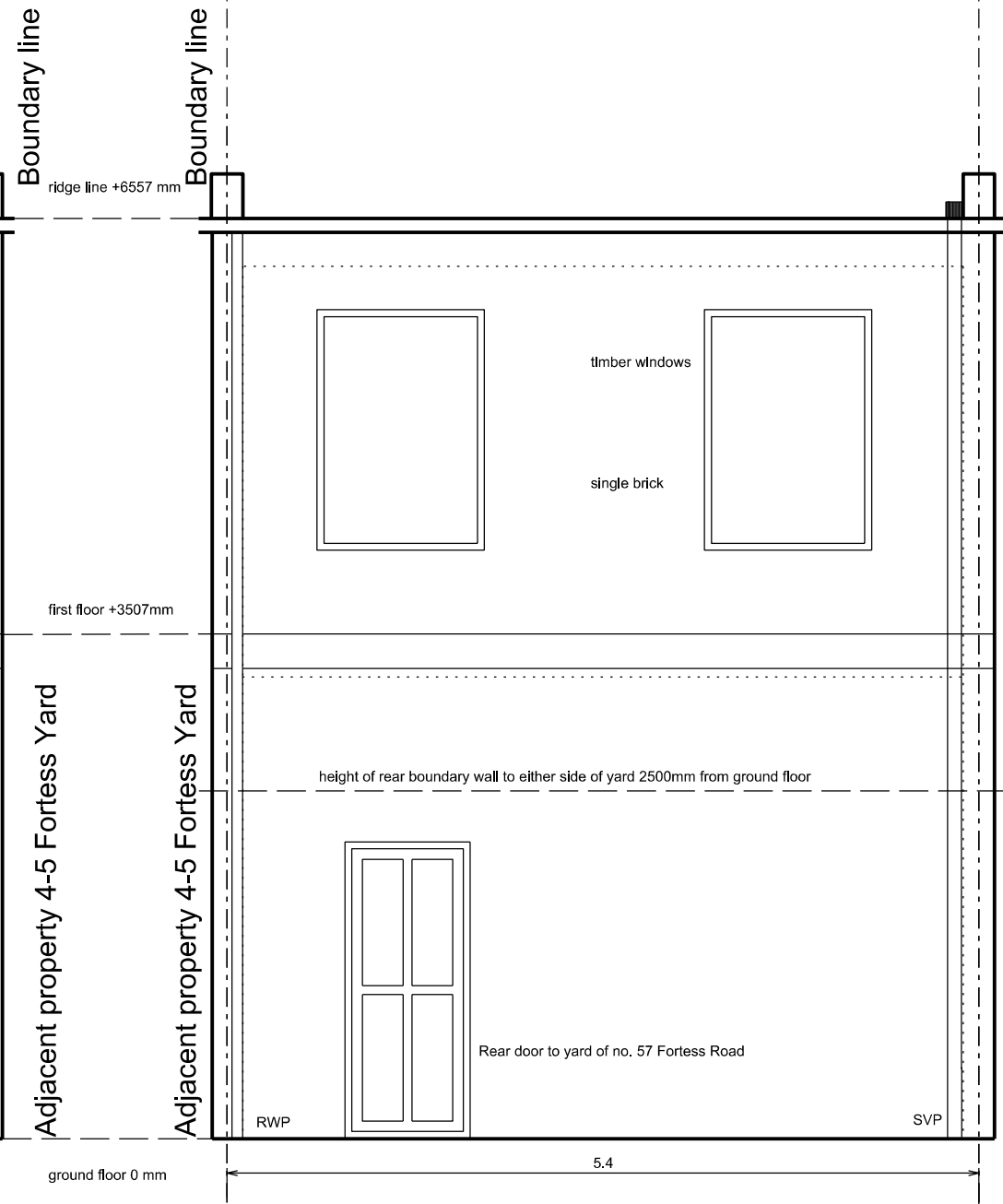
REAR ELEVATION
