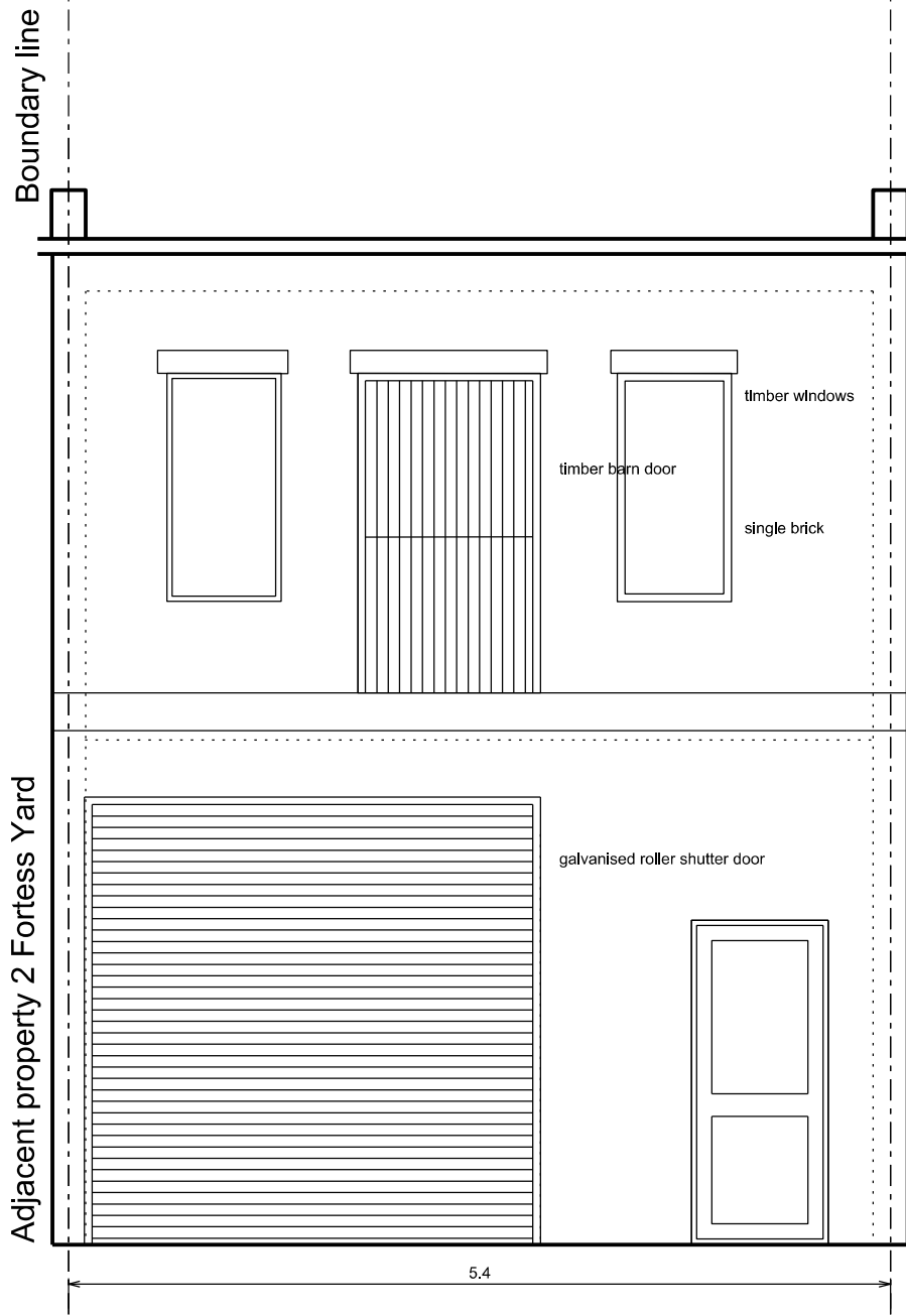
FRONT ELEVATION
