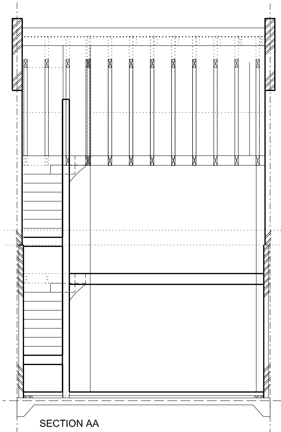
PROPOSED SECTIONS 3 Fortress Yard London NW5
