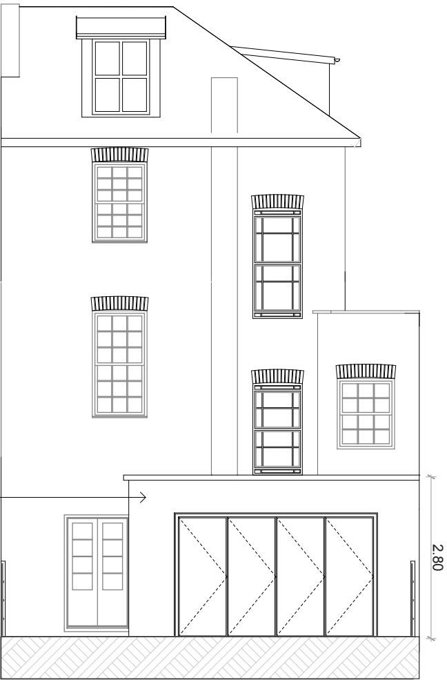
Rear Elevation 1:100
