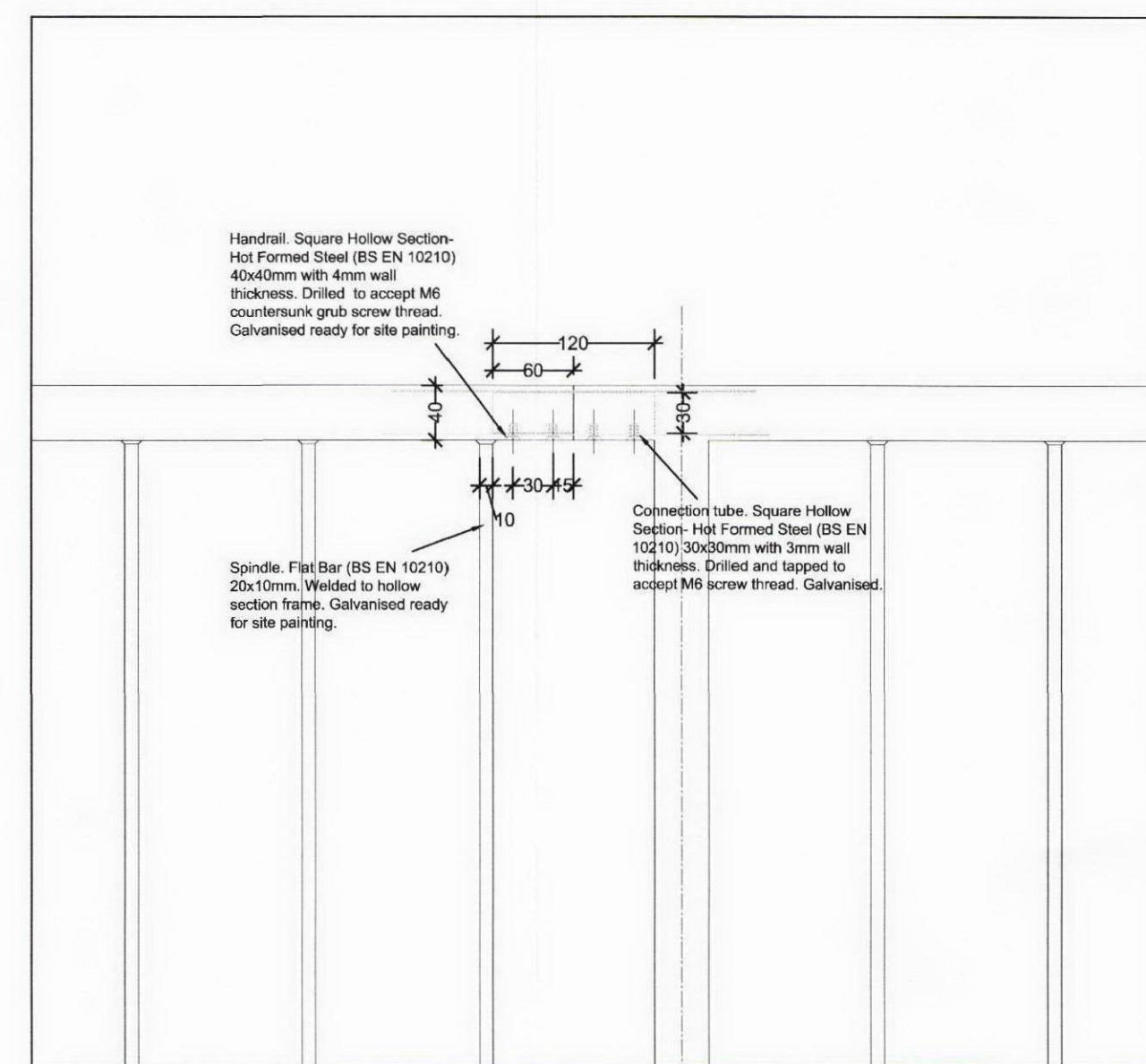
Connection Detail 1:5
