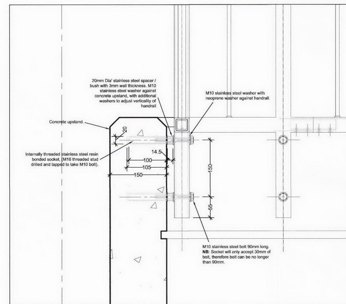
Fixing Detail 1:5
