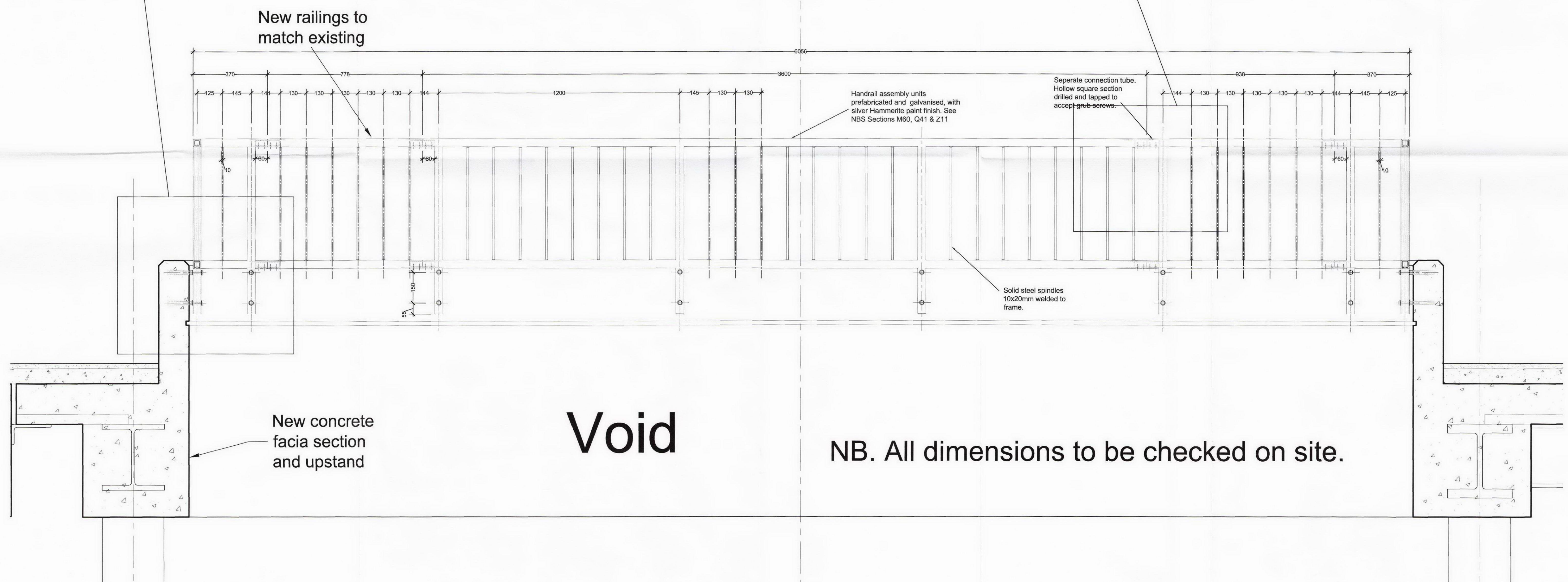
East - West Section 1:10
