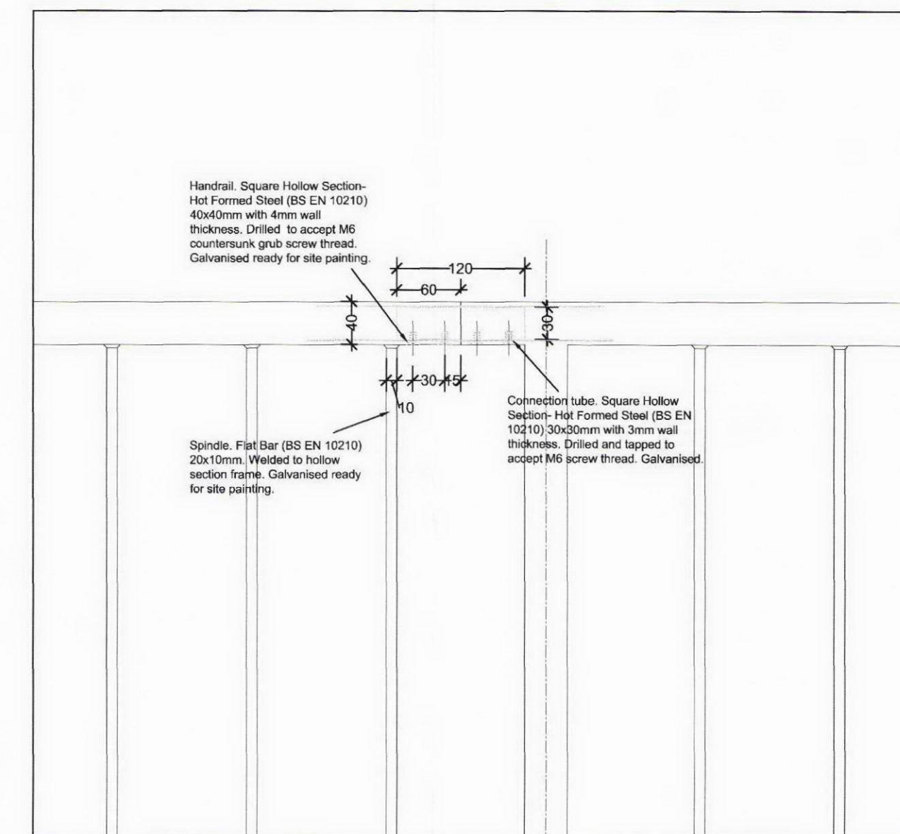
Connection Detail 1:5
