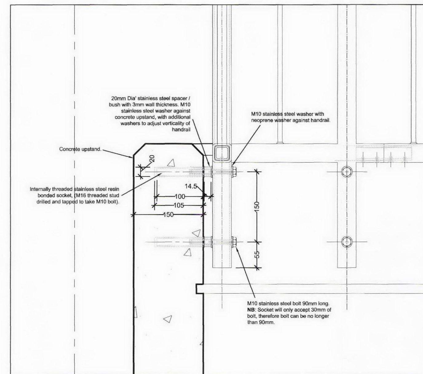
Fixing Detail 1:5
