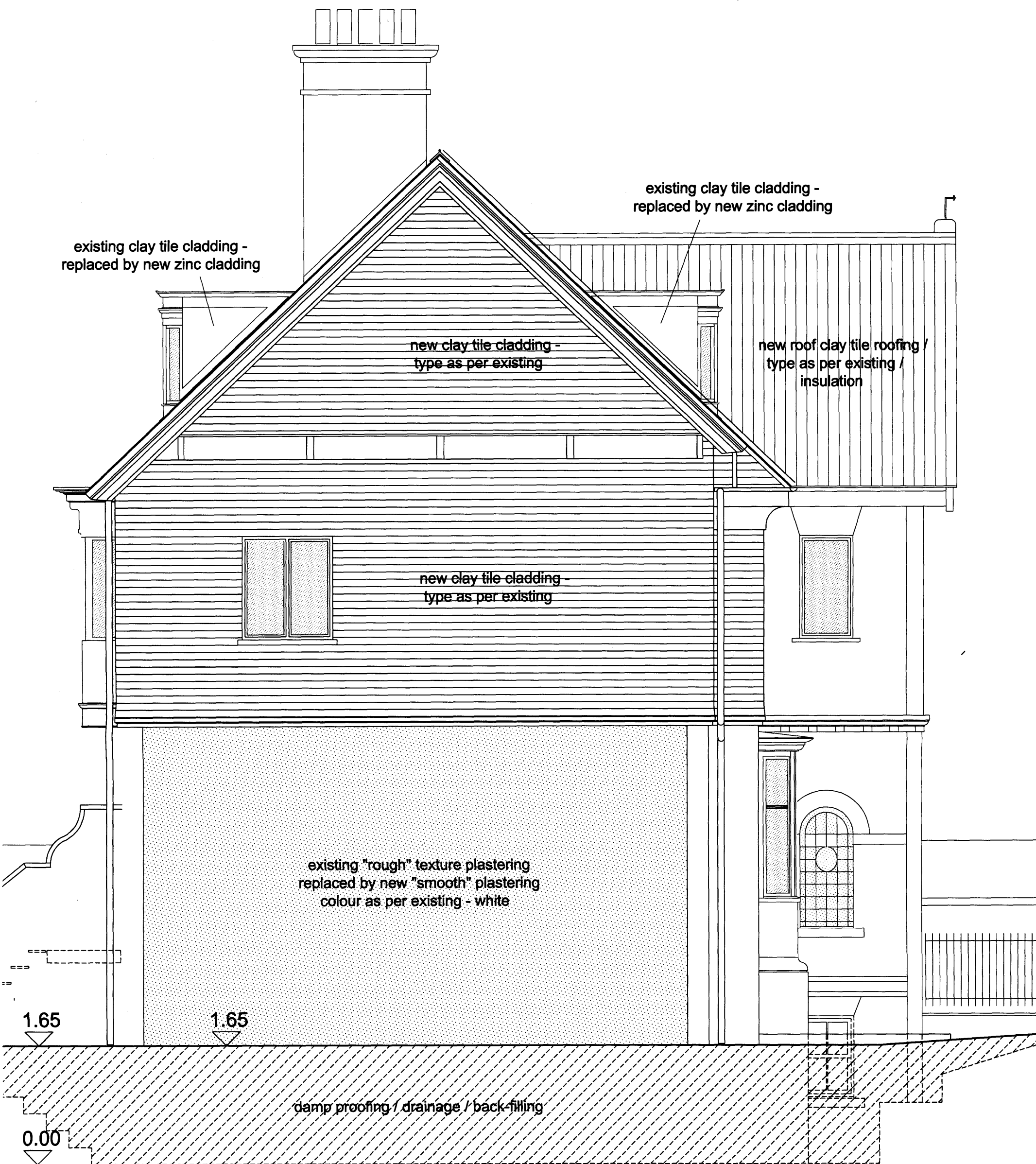
Facade - Gable 1
