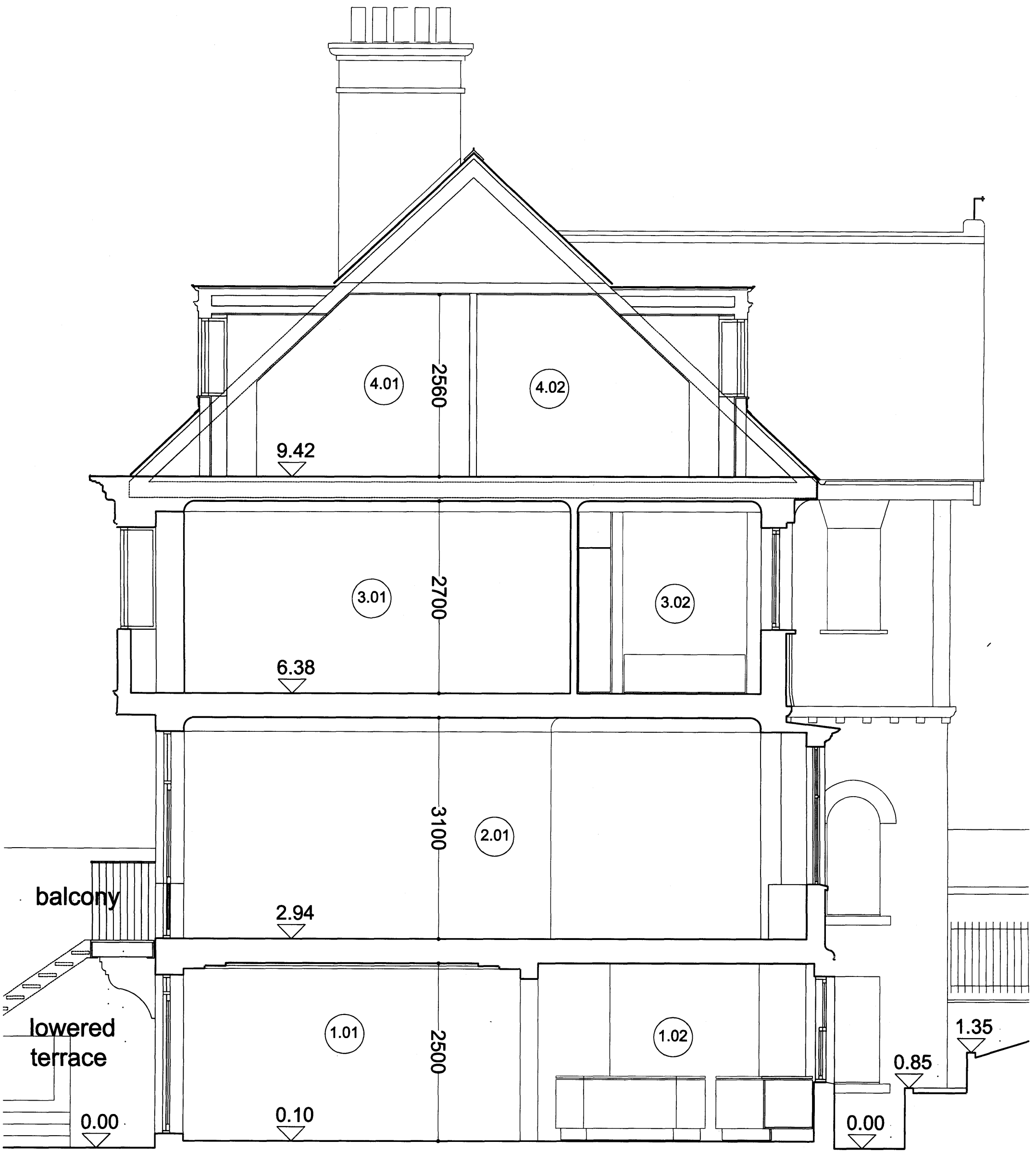
Existing Cross Section - Existing
