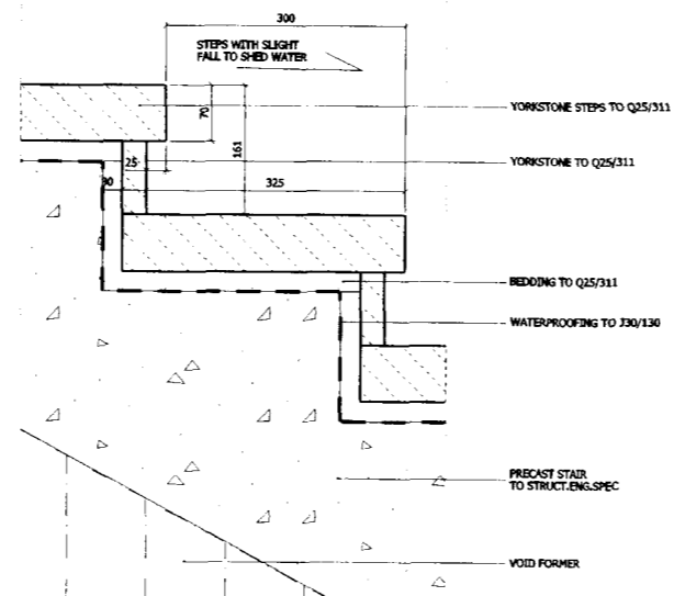
03 STAIR TO RESI PODIUM - TYPICAL BUILD UP (ON PRECAST STAIR) 05070_GA_Elev_Balc_GG_01.dgn
