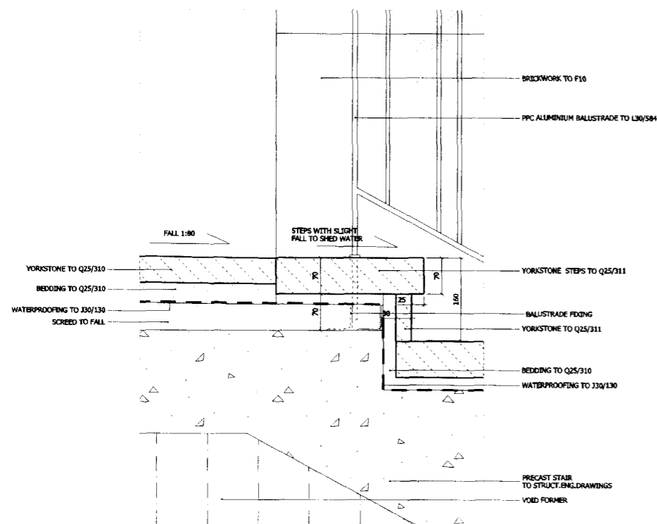
02 TYPICAL DETAIL - BALUSTRADE FIXING 05070_GA_Elev_Balc_GG_01.dgn
