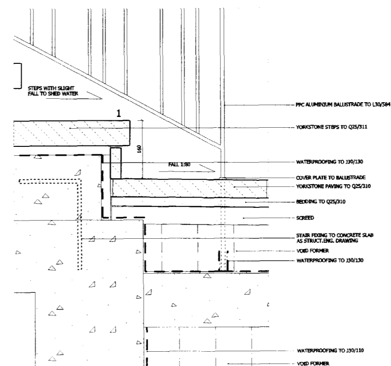
04 STAIR TO RESI PODIUM - BALUSTRADE FIXING 05070_GA_Elev_Balc_GG_01.dgn
