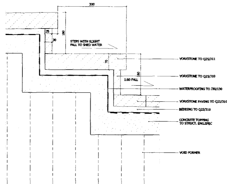
01 TYPICAL PODIUM STAIR DETAIL (ON VOID FORMER) 05070_BDW_Sect_WW_01.dgn
