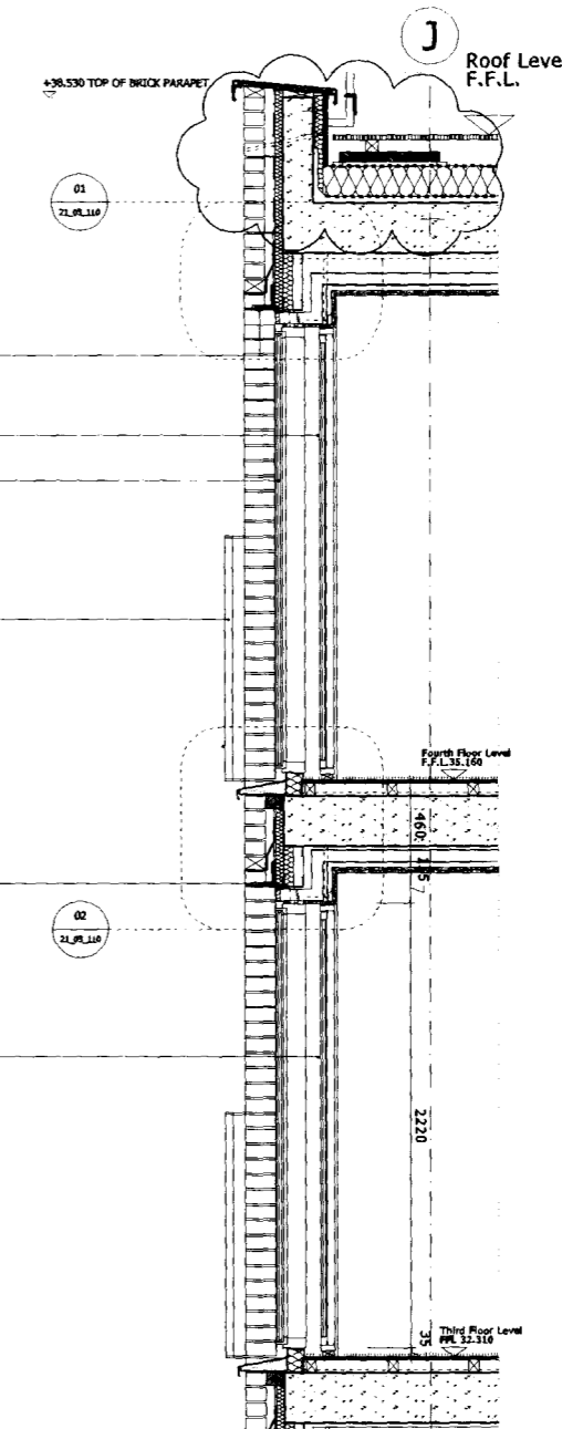
03 Vertical Section 05070_GA_Elev_VSec_01.dgn
