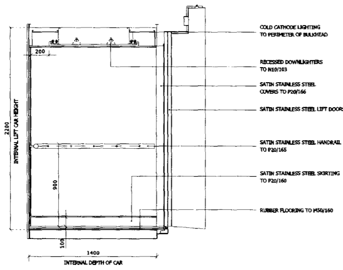
04 Side Elevation 05070_InWks_Lift_Car_BlkC_01.dgn
