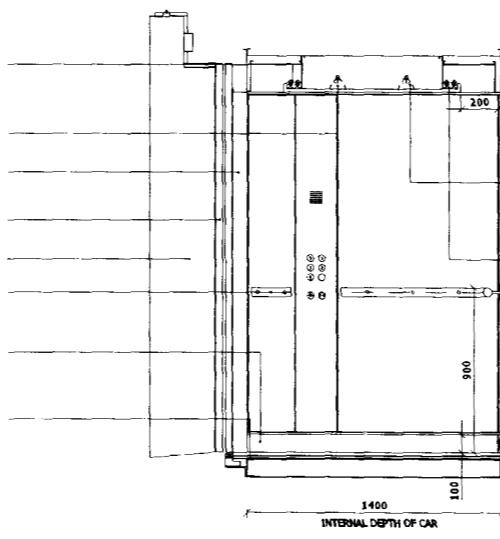
05 Control Side Elevation 05070_InWks_Lift_Car_BlkC_01.dgn
