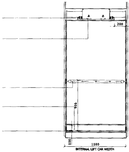
02 Rear Elevation 05070_InWks_Lift_Car_BlkC_01.dgn
