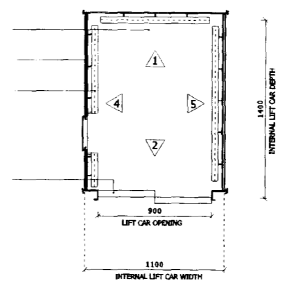
03 Floor Plan 05070_InWks_Lift_Car_BlkC_01.dgn
