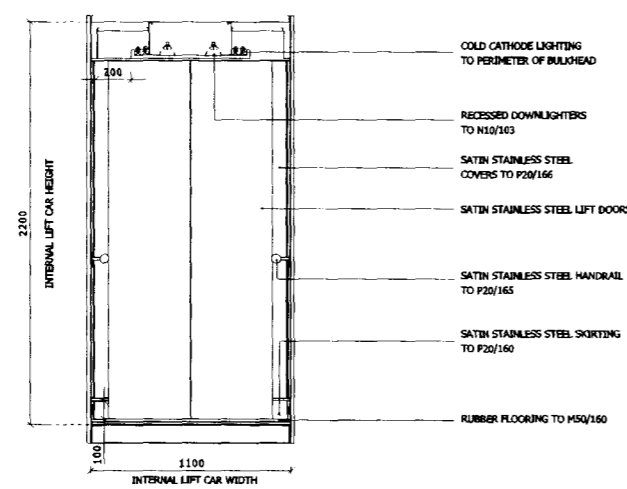
01 Front Elevation 05070_InWks_Lift_Car_BlkC_01.dgn
