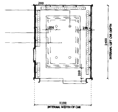
06 Reflected Ceiling Plan 05070_InWks_Lift_Car_BlkC_01.dgn
