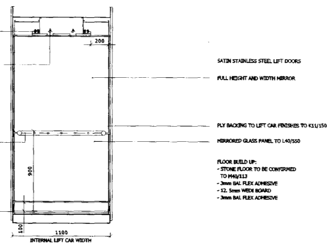
02 Rear Elevation 05070_InWks_Lift_Car_BkC_01.dgn
