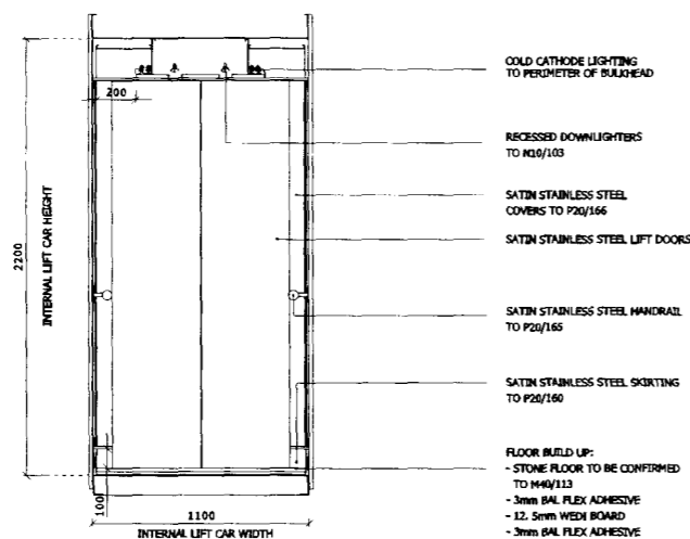
01 Front Elevation 05070_InWks_Lift_Car_BkC_01.dgn
