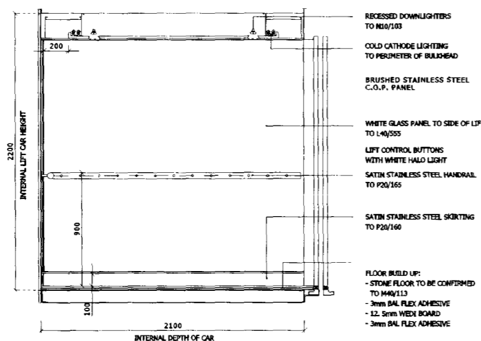
04 Side Elevation 05070_InWks_Lift_Car_BkC_01.dgn
