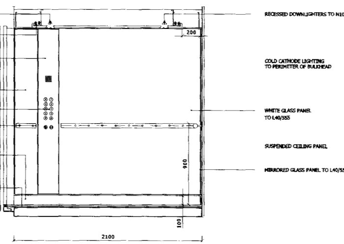
05 Control Side Elevation 05070_InWks_Lift_Car_BkC_01.dgn
