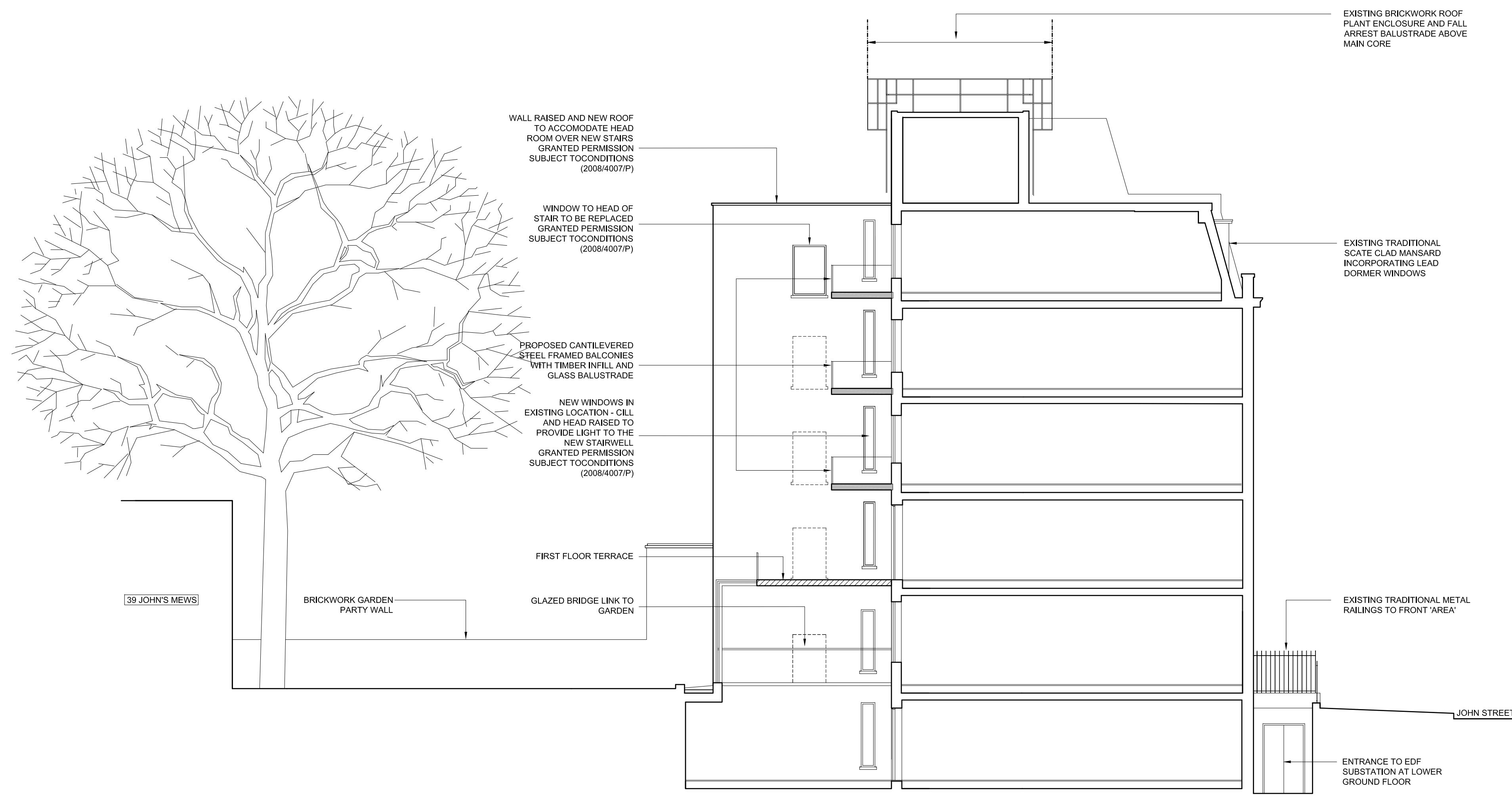
NORTH COURTYARD ELEVATION / SEC AA
