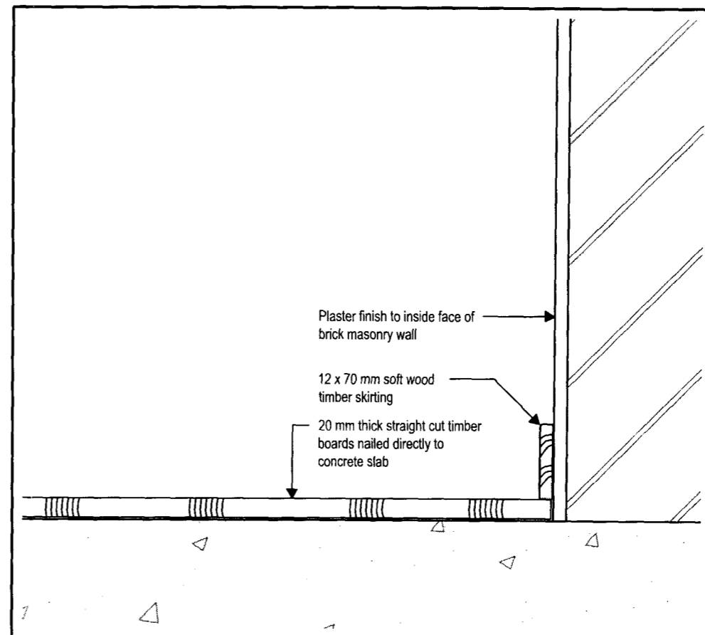
Skirting Detail - Existing
