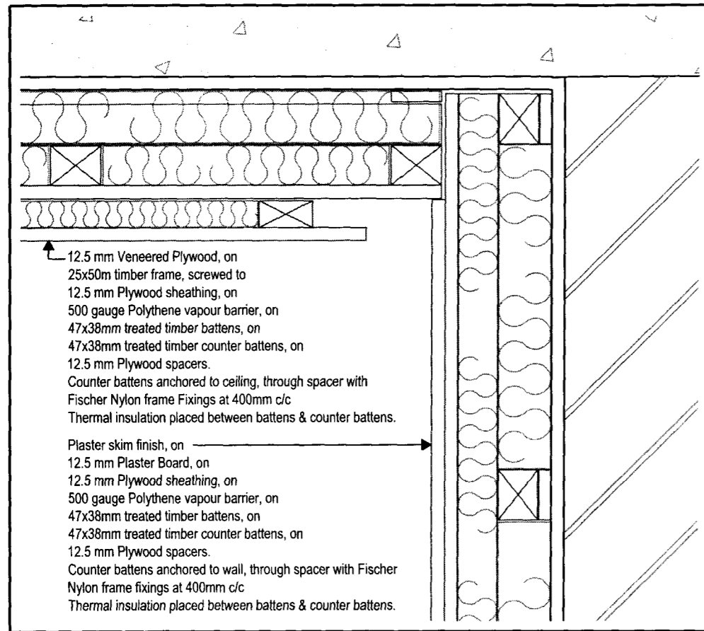
Wall Head Detail - Proposed
