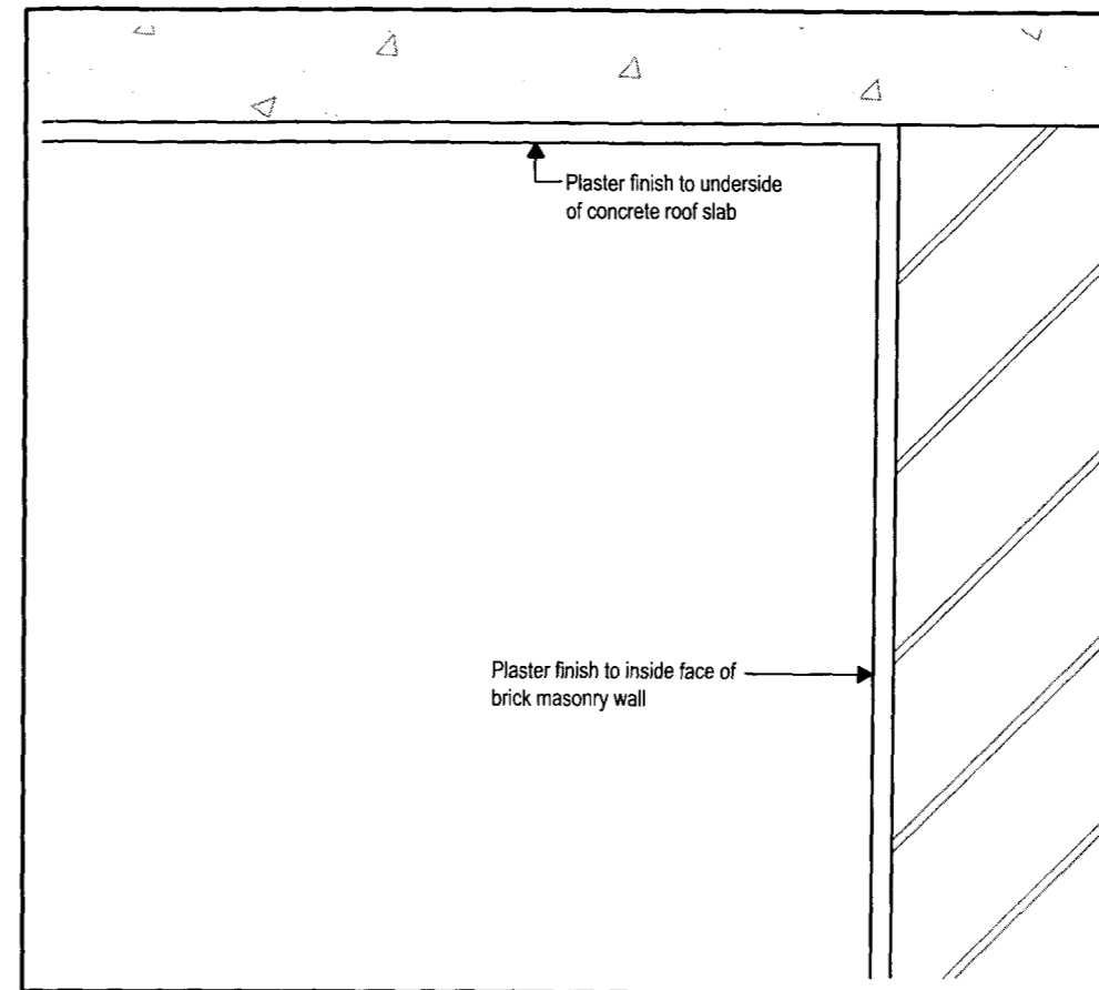
Wall Head Detail - Existing
