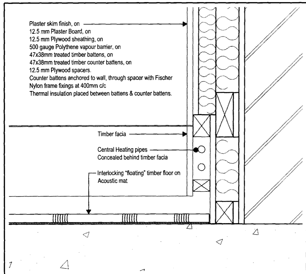
Skirting Detail - Proposed
