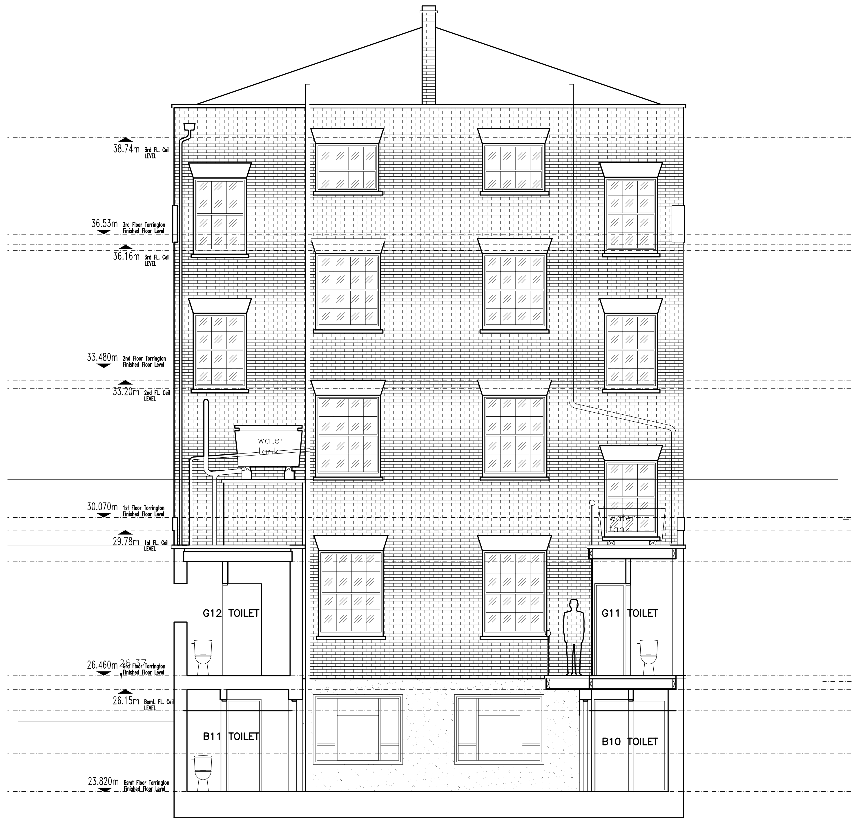
TORRINGTON PLACE EXISTING SECTION/ELEVATION 2-2
