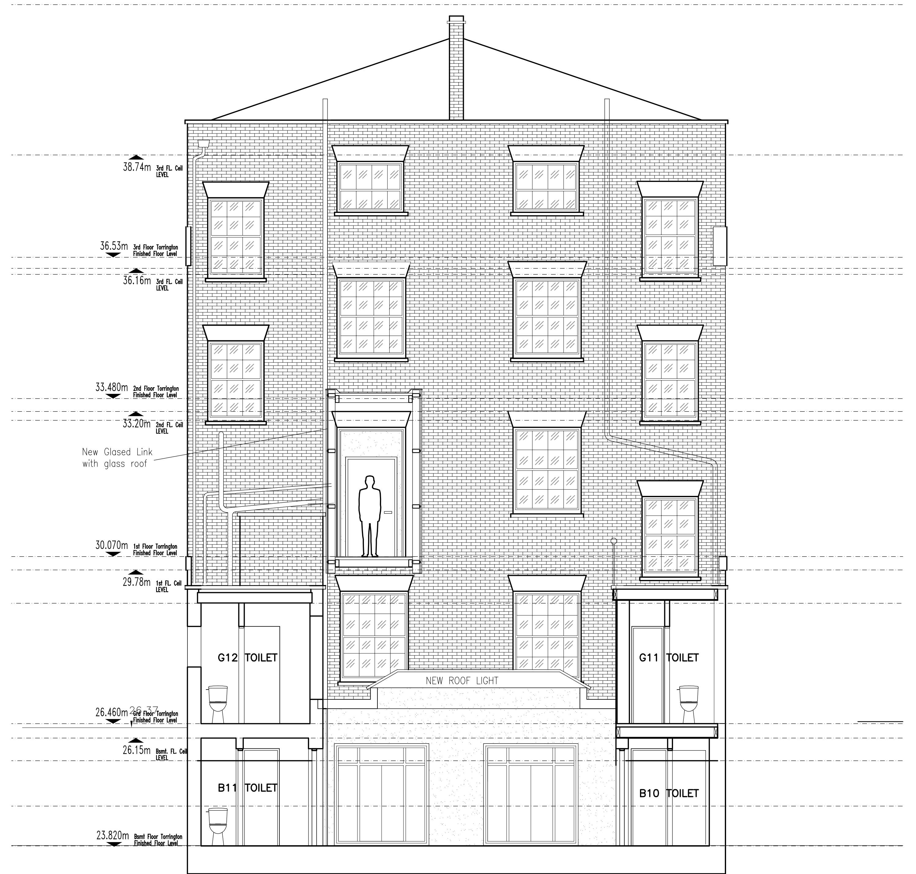
TORRINGTON PLACE PROPOSED SECTION/ELEVATION 2-2
