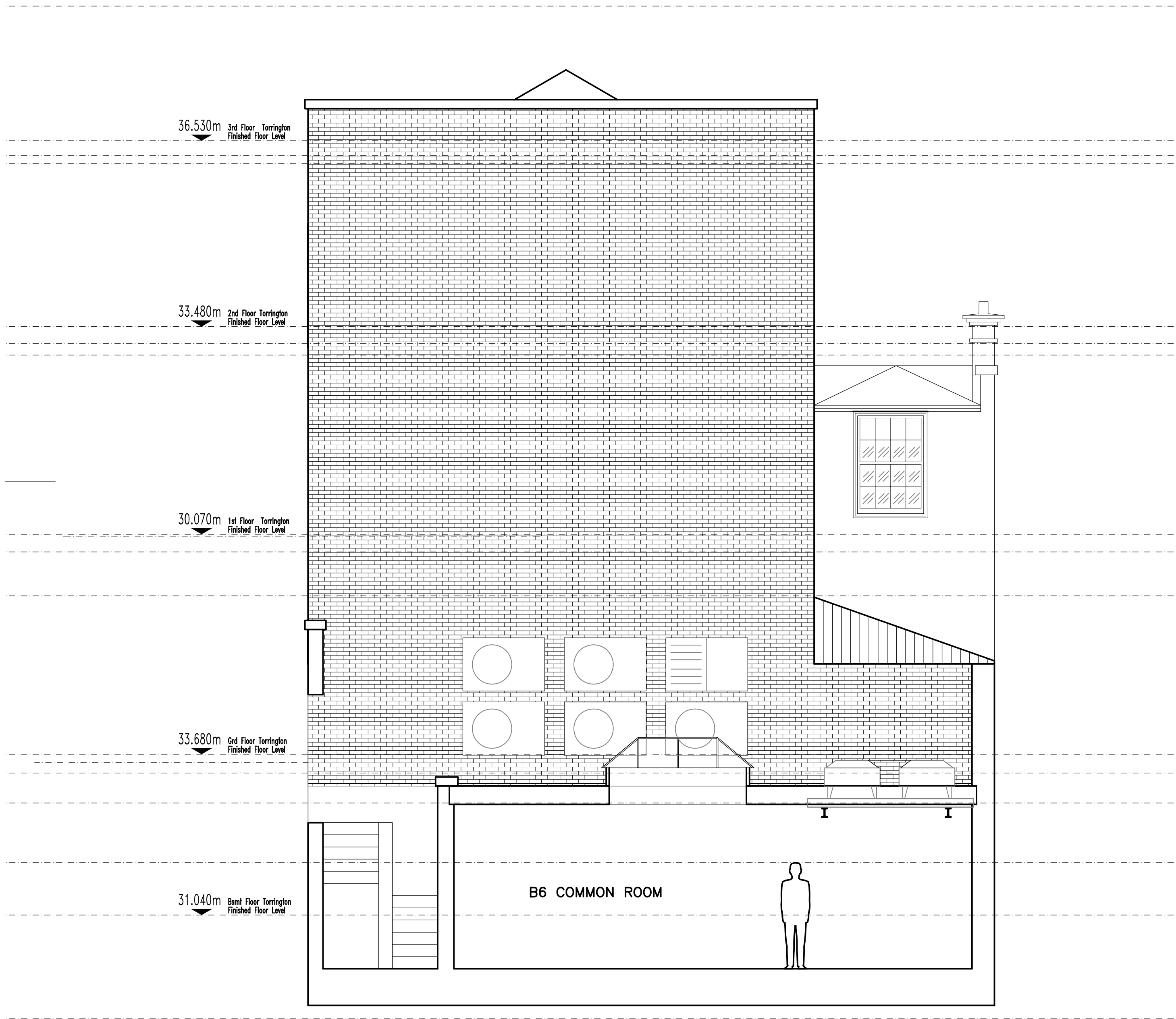
TORRINGTON PLACE EXISTING SECTION/ELEVATION 1-1
