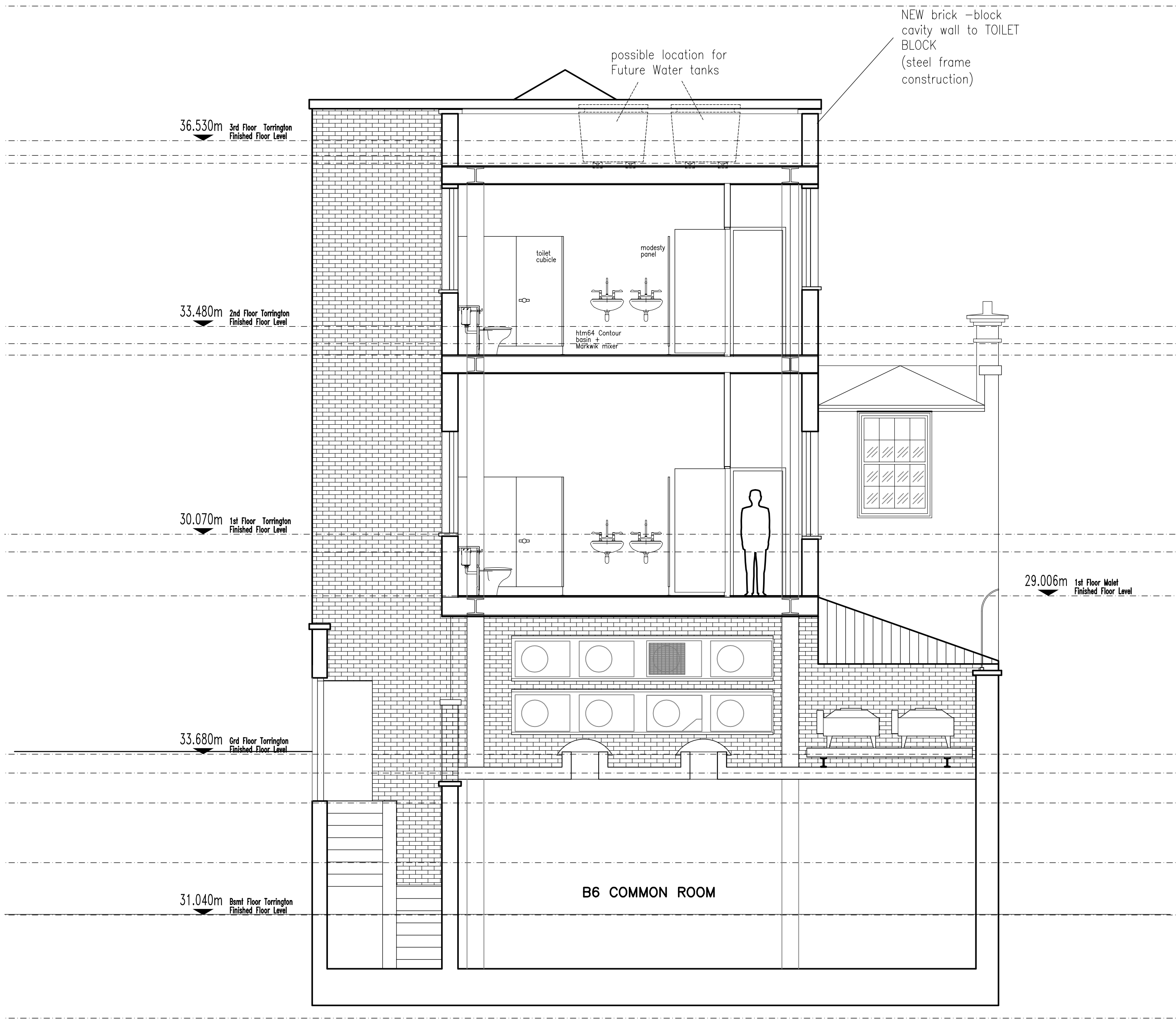
TORRINGTON PLACE PROPOSED SECTION/ELEVATION 1-1
