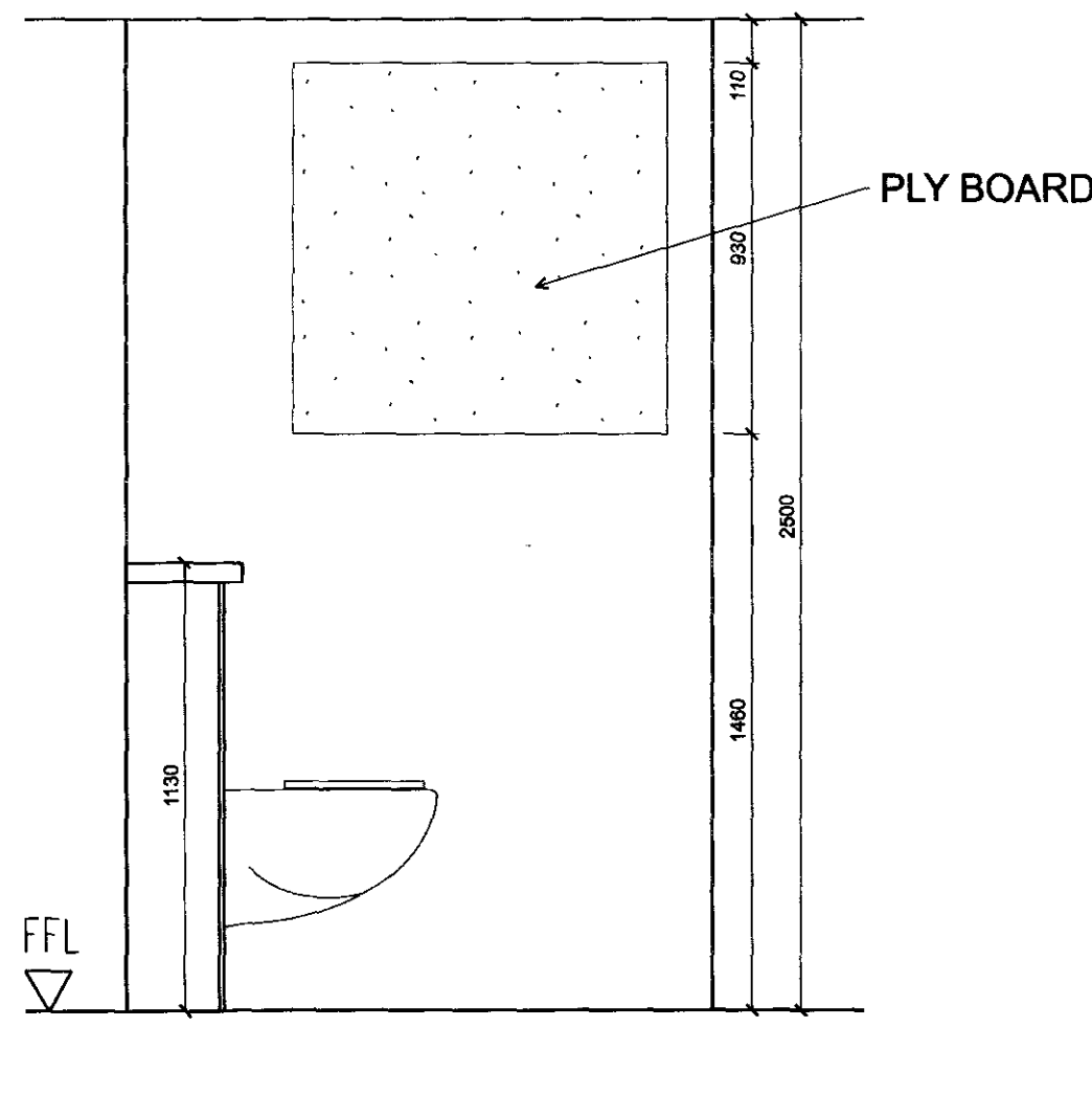
4 ELEVATION BB FIRST FLOOR
