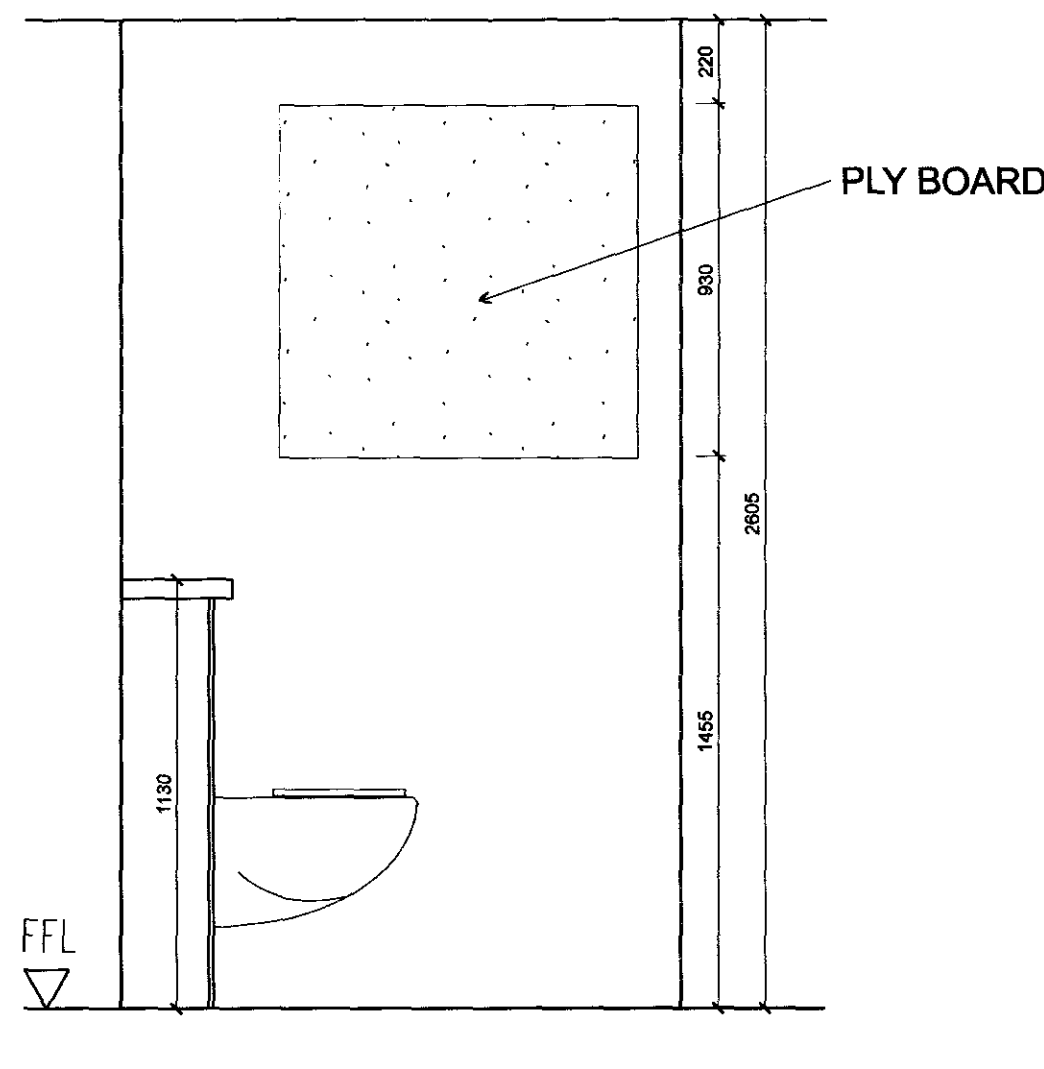
6 ELEVATION CC GROUND FLOOR
