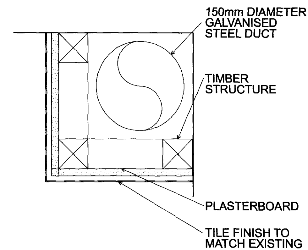
14 STEEL DUCT TYPICAL DETAIL
