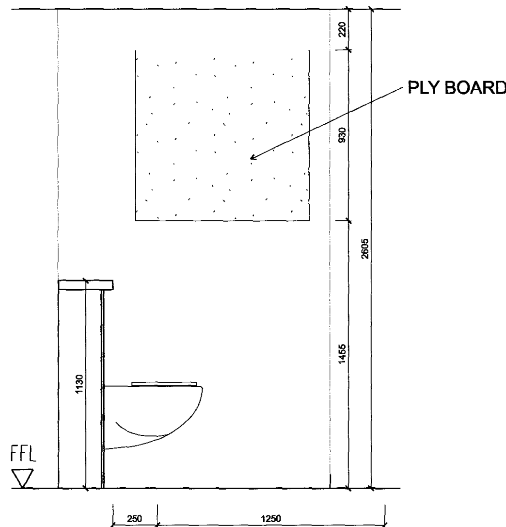
2 ELEVATION AA SECOND FLOOR
