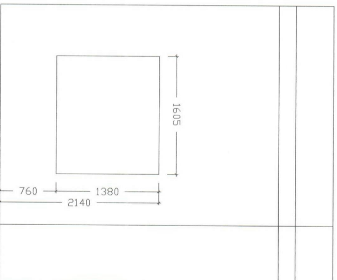
Proposed Elevation
