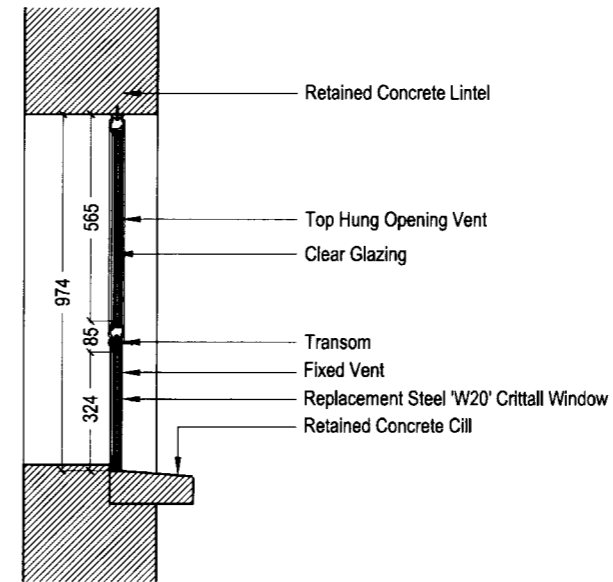
Proposed Section
