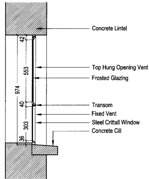
Existing Section
