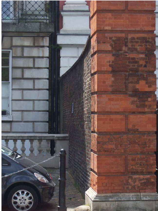
6. Bowing and leaning of the south wall.
