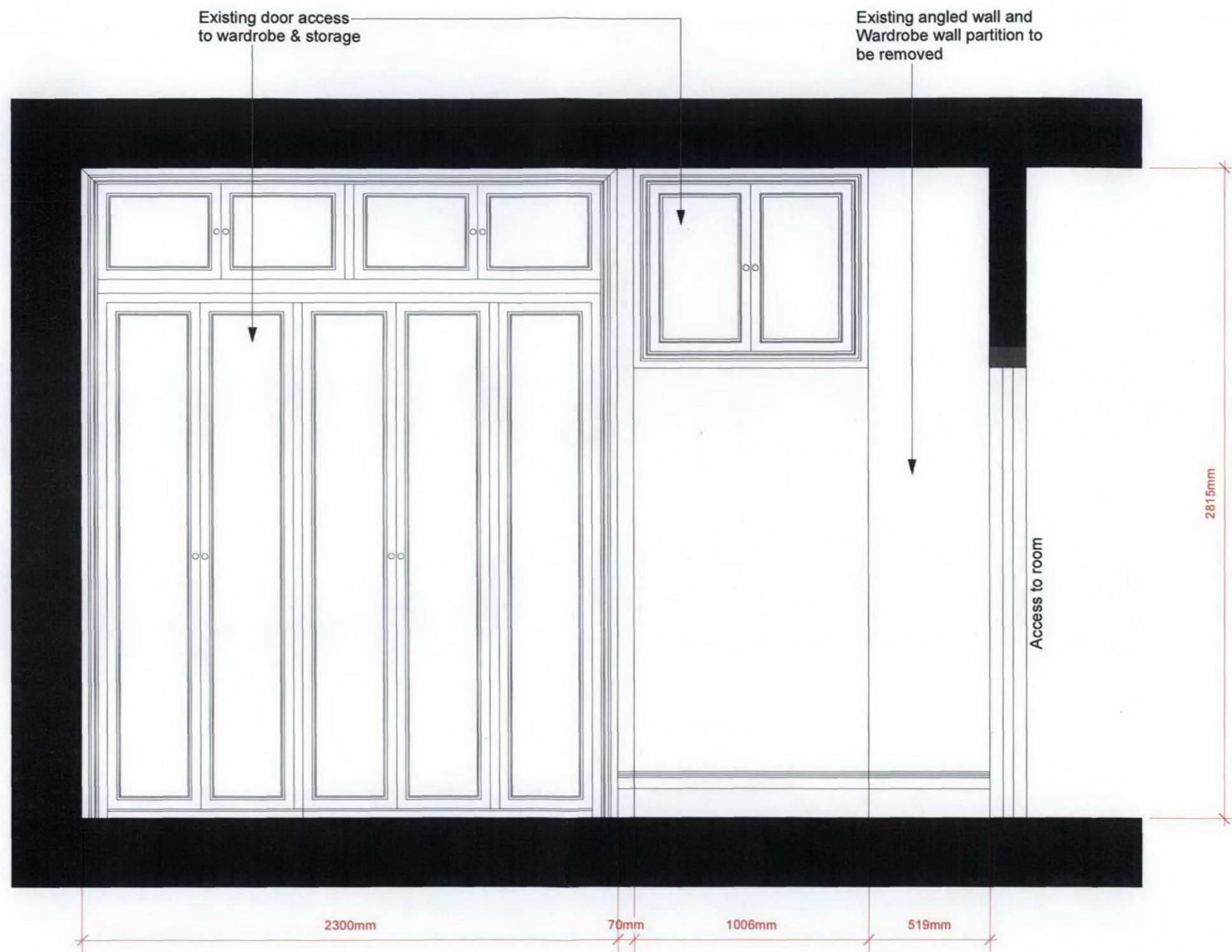
Elevation 2 - Master Bedroom
